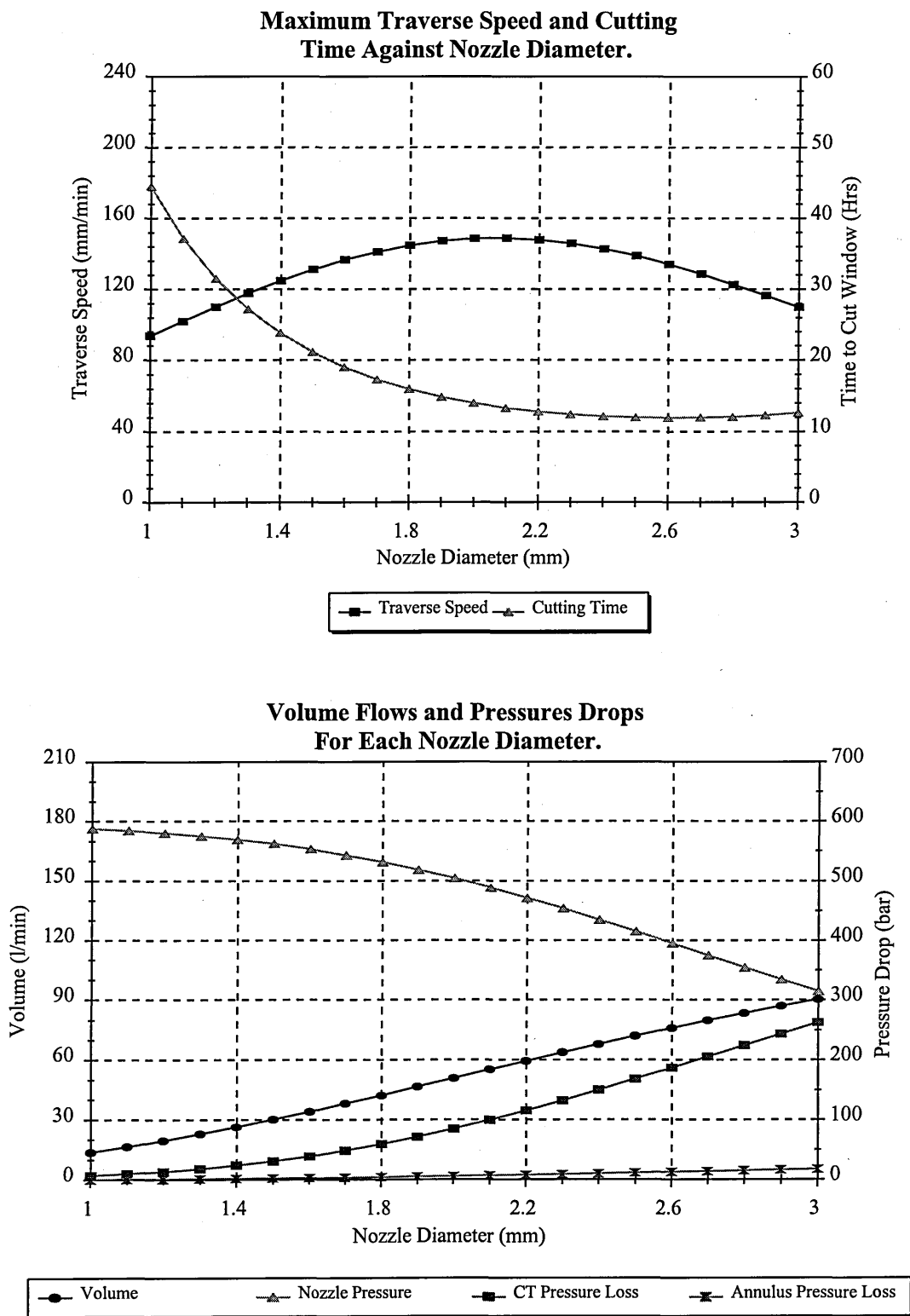
GRAPH 5.4.1 TYPICAL RESULTS FROM THE OPTIMISATION PROGRAM FOR 1 NOZZLE
