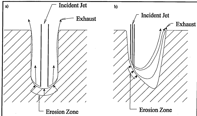
FIGURE 2.3.1 COMPARISON OF THE MATERIAL MOVING MECHANISMS: a) for a stationary jet and b) for a moving jet.
