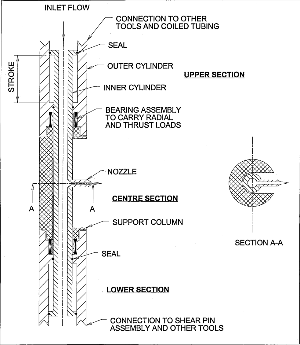
FIGURE 7.3.1 PRESSURE BALANCED TELESCOPIC SECTION WITH SUPPORT COLUMN
