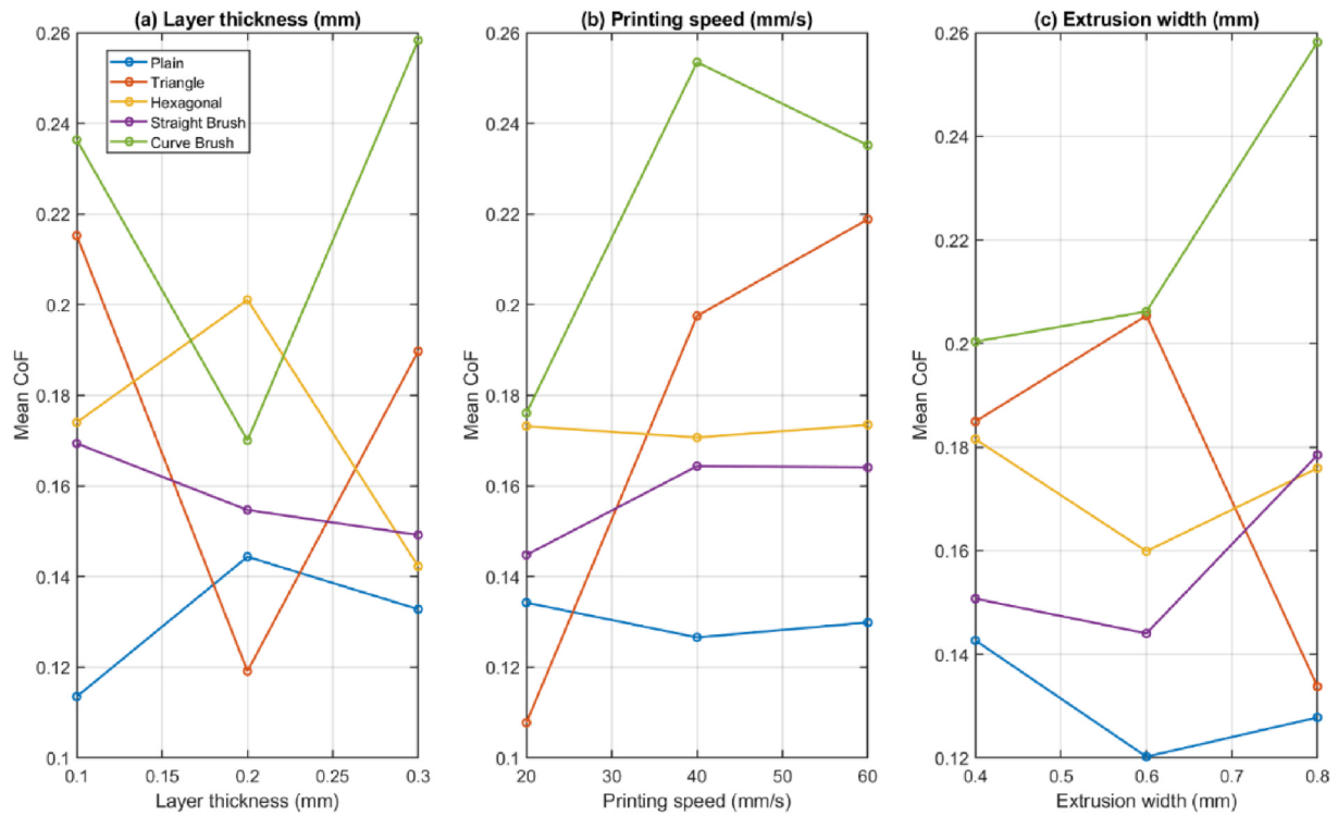
Fig. 5. Effects of printing parameters on CoF for different surface structures.
