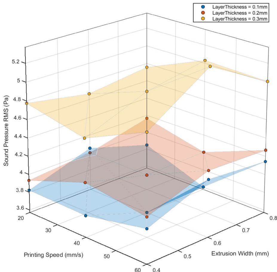
Fig. 9. Response surface of the sound pressure of the Plain surface as a function of printing speed and extrusion width at different layer thickness levels.
