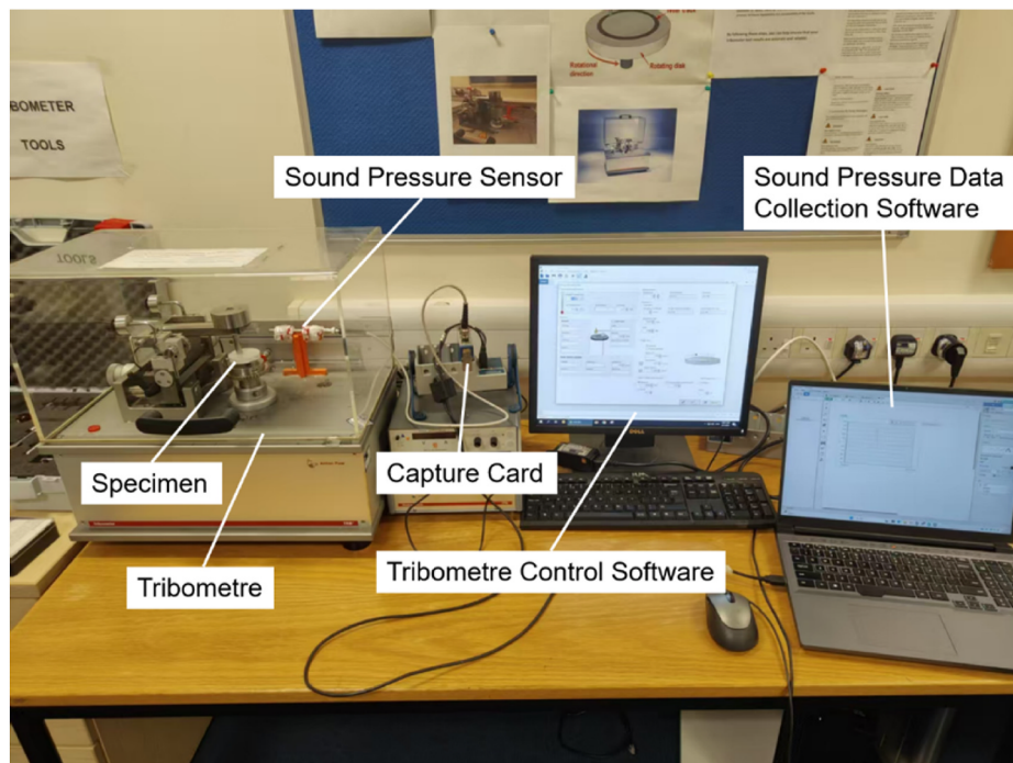
Fig. 3. Experimental setup.
