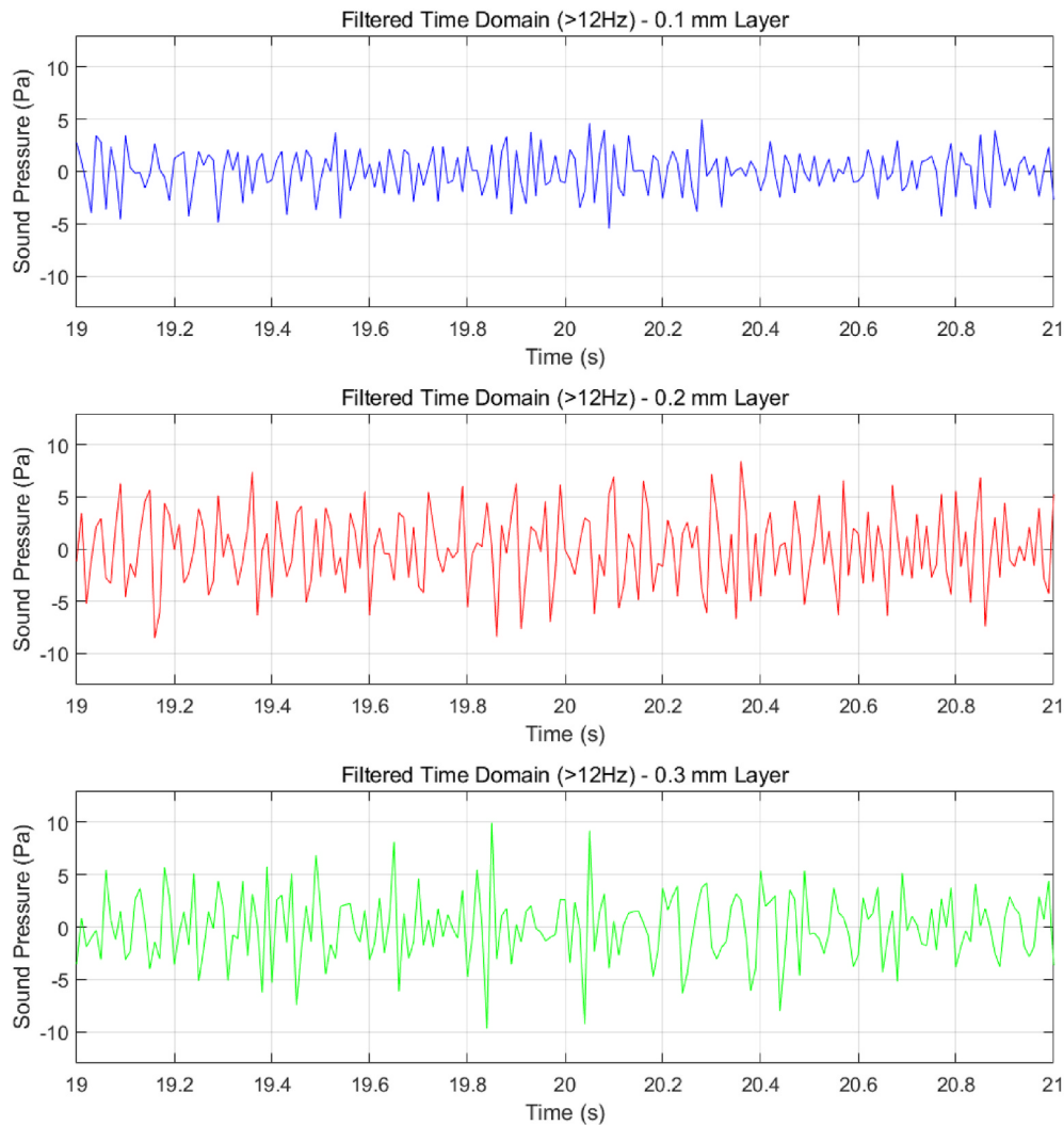
Fig. 13. Zoomed-in filtered time-domain waveforms within the 19–21 s interval.
