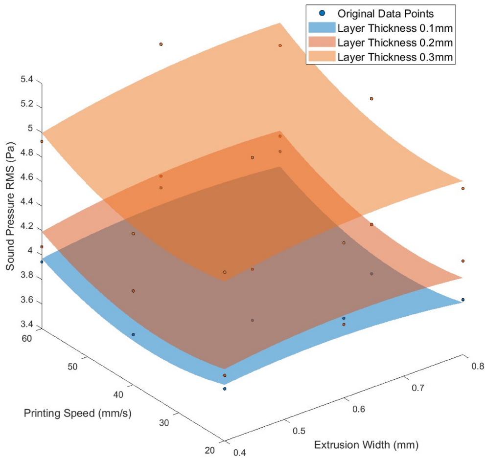
Fig. 16. Fitted response surfaces illustrating the effect of printing speed and extrusion width on the RMS sound pressure of the Plain surface at different layer thickness levels (0.1, 0.2, and 0.3 mm). The markers represent the original experimental data points.
