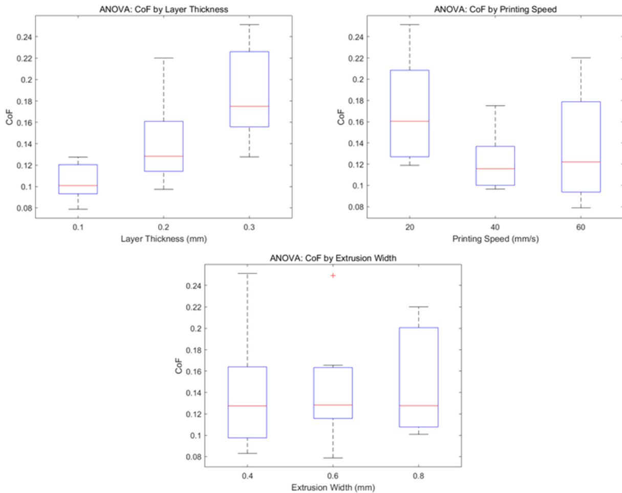
Fig. 8. ANOVA of the CoF for the Plain surface with respect to (a) layer thickness, (b) printing speed, and (c) extrusion width.
