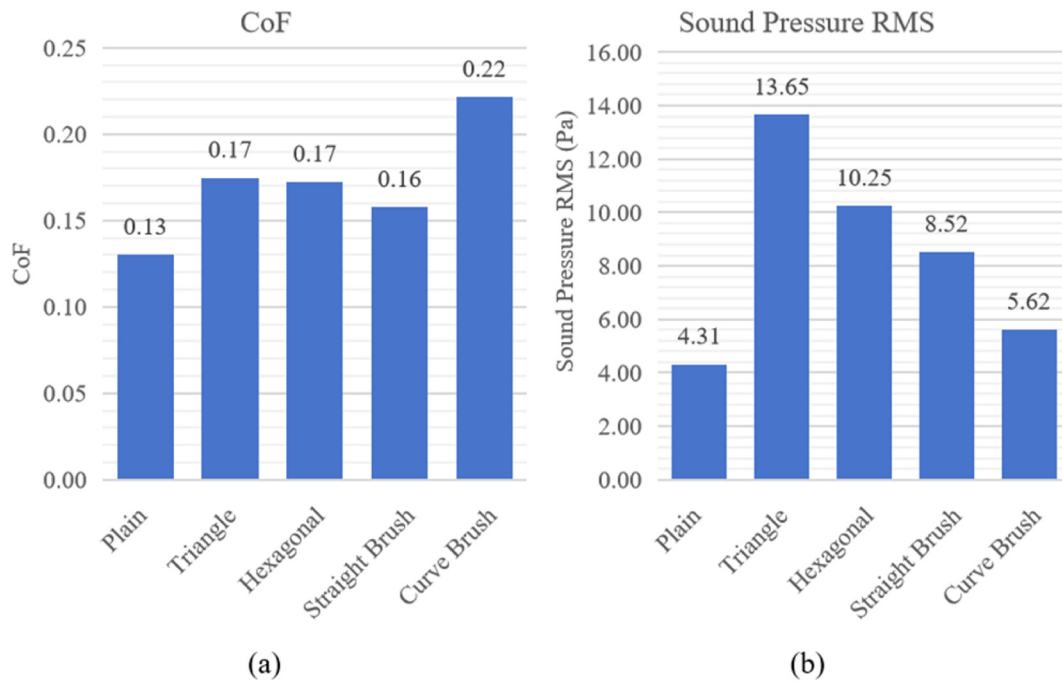
Fig. 4. Mean CoF and RMS sound pressure of different surface designs.
