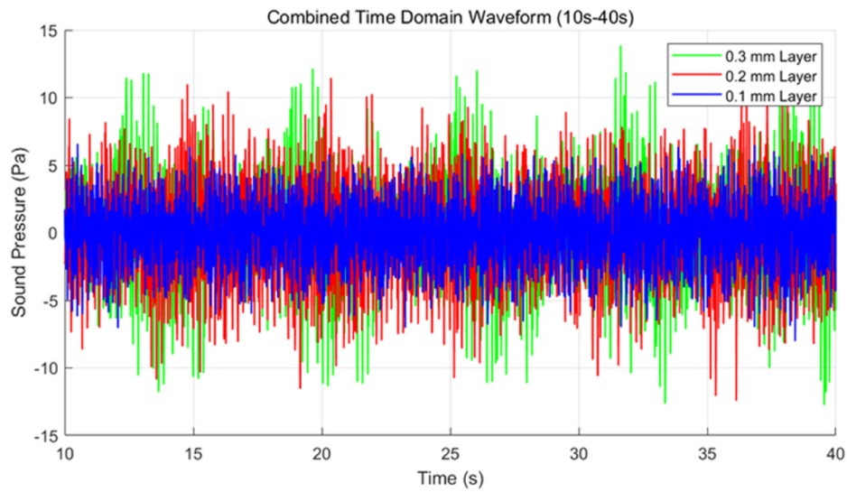
Fig. 11. Time-domain waveforms of friction noise (10–40 s) for three different layer thicknesses.
