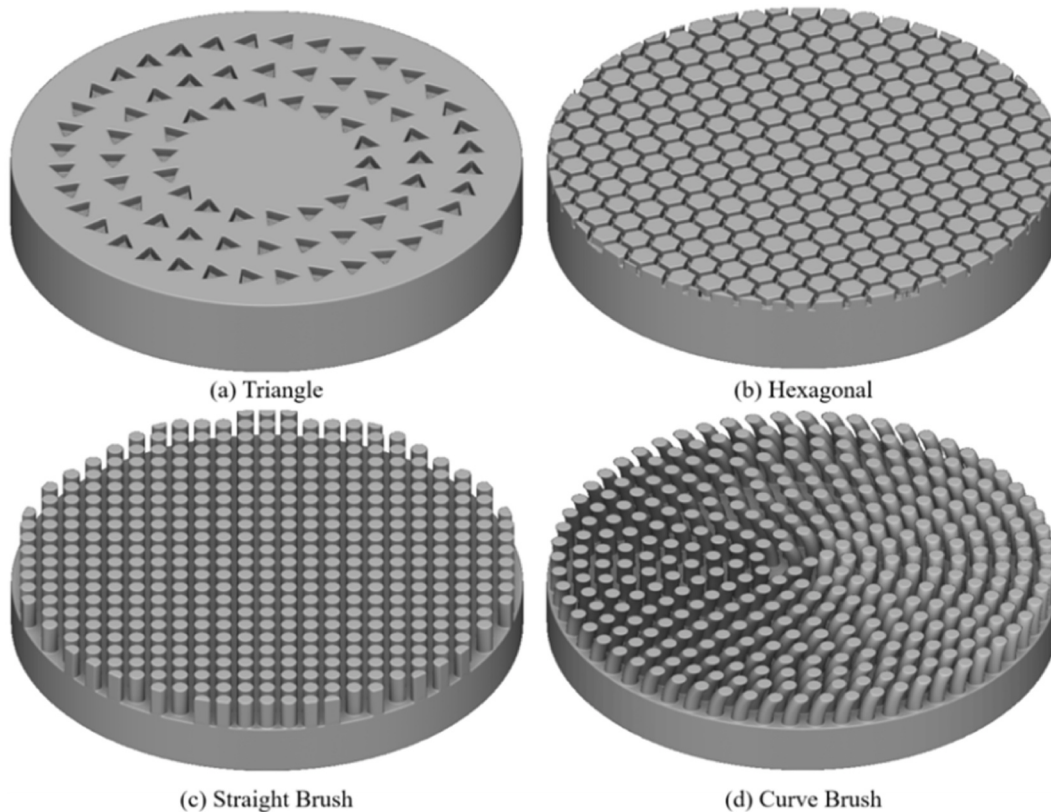
Fig. 2. Surface-structure geometries (dimensions in mm). (a) Triangle: three circumferential rings of equilateral triangular pits inscribed in 3-mm circles at radii 10, 15, and 20; depth 1. (b) Hexagonal: periodic array of regular hexagonal protrusions, side length 1.75, height 0.5, spacing 0.5. (c) Brush (straight): periodic array of cylindrical posts, diameter 1.5, height 3, spacing 2. (d) Curved brush: circumferentially oriented curved cylindrical posts generated by sweeping a 1.5-mm-diameter circle along an arc; height 3.
