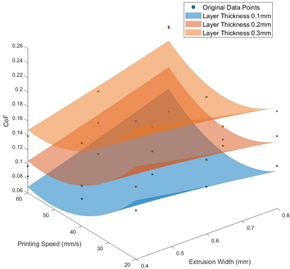
Fig. 15. Fitted response surfaces illustrating the effect of printing speed and extrusion width on the CoF of the Plain surface at different layer thickness levels (0.1, 0.2, and 0.3 mm). The markers represent the original experimental data points.
