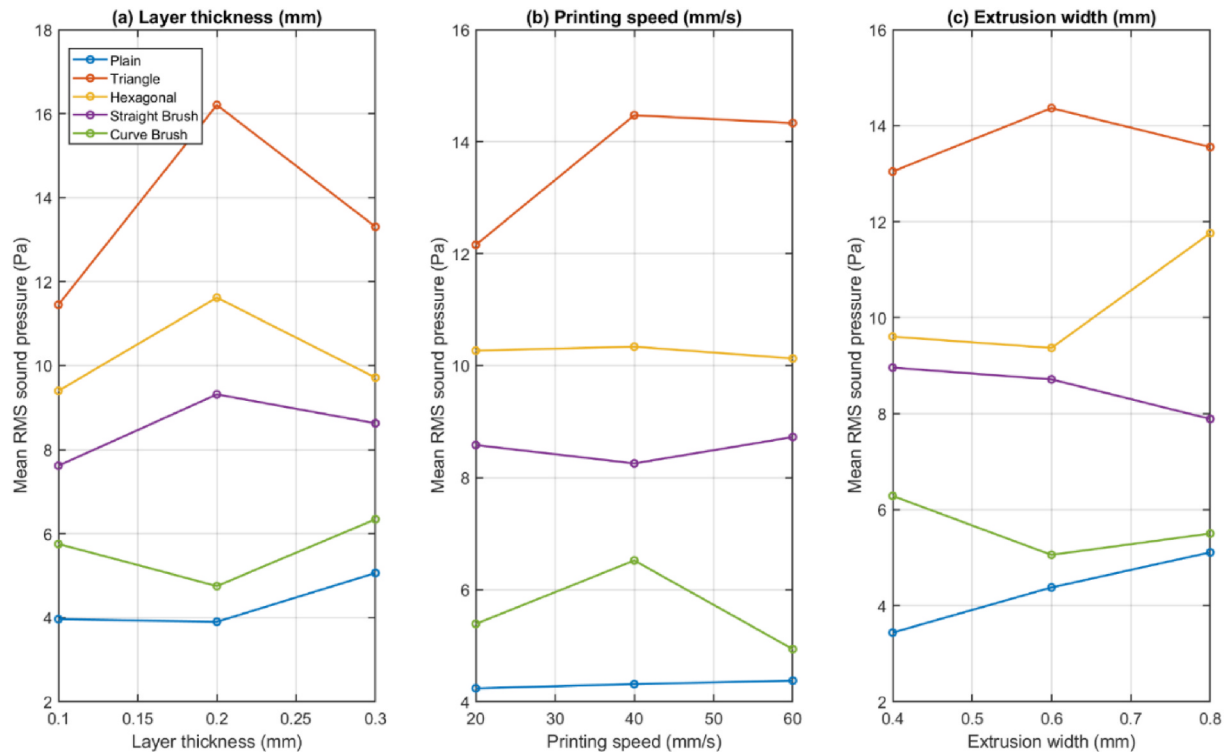
Fig. 6. Effects of printing parameters on RMS sound pressure for different surface structures.
