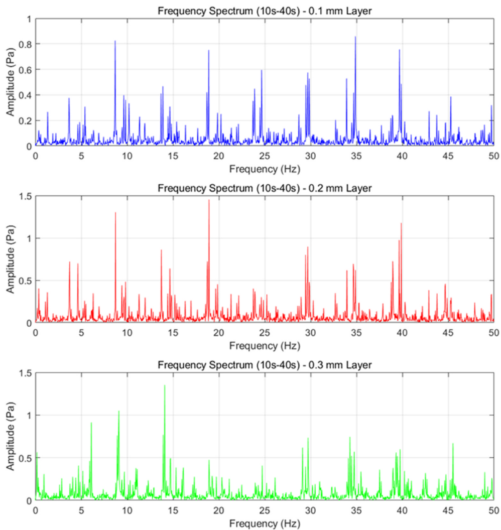
Fig. 12. FFT frequency-domain spectra for three different layer thicknesses.
