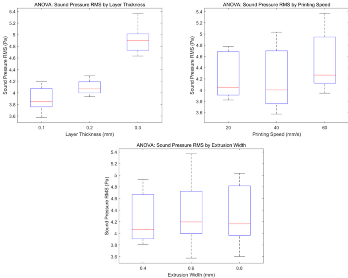
Fig. 10. ANOVA of the sound pressure for the Plain surface with respect to (a) layer thickness, (b) printing speed, and (c) extrusion width.
