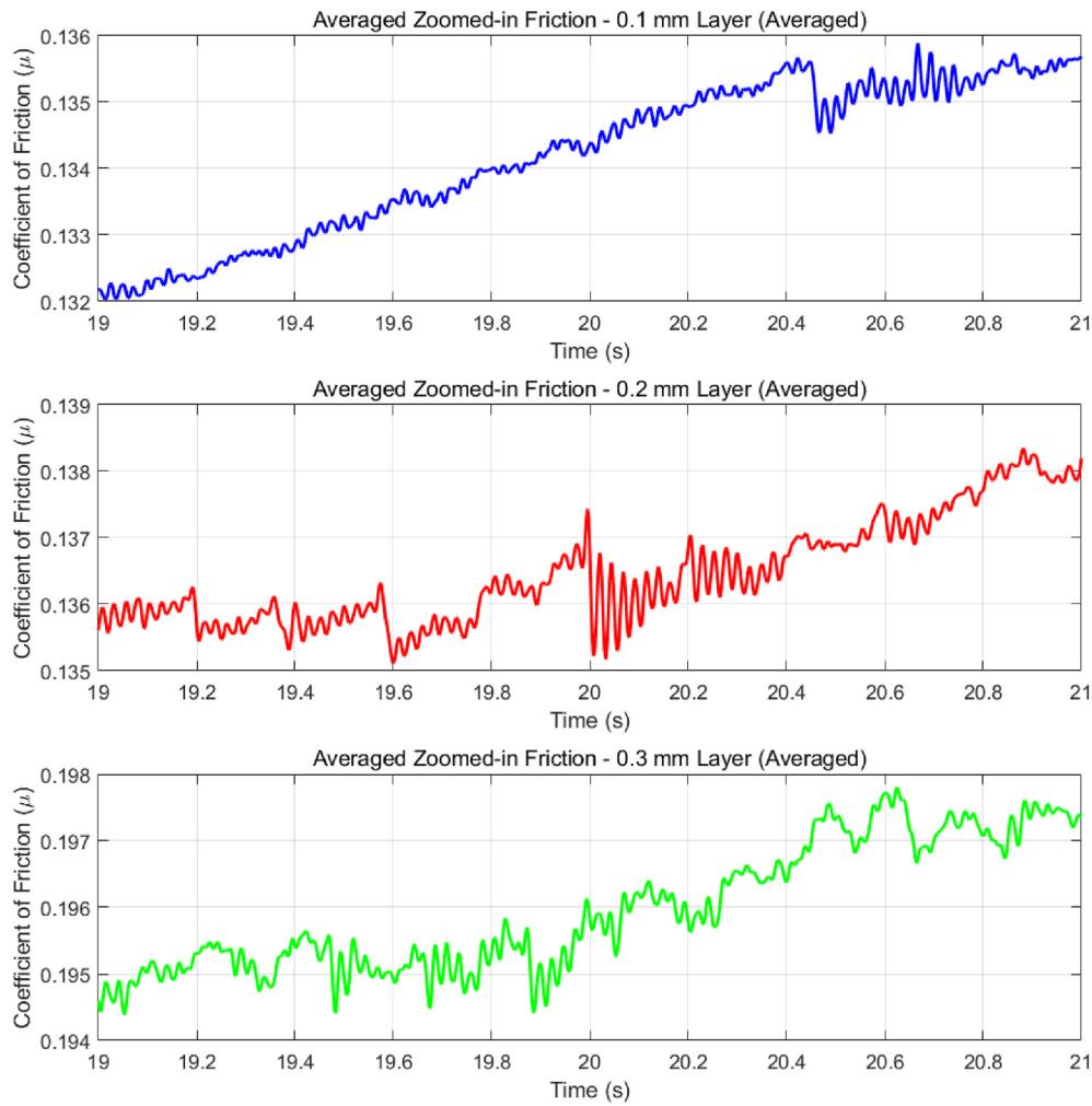
Fig. 14. Zoomed-in friction coefficient curves within the 19–21 s interval.
