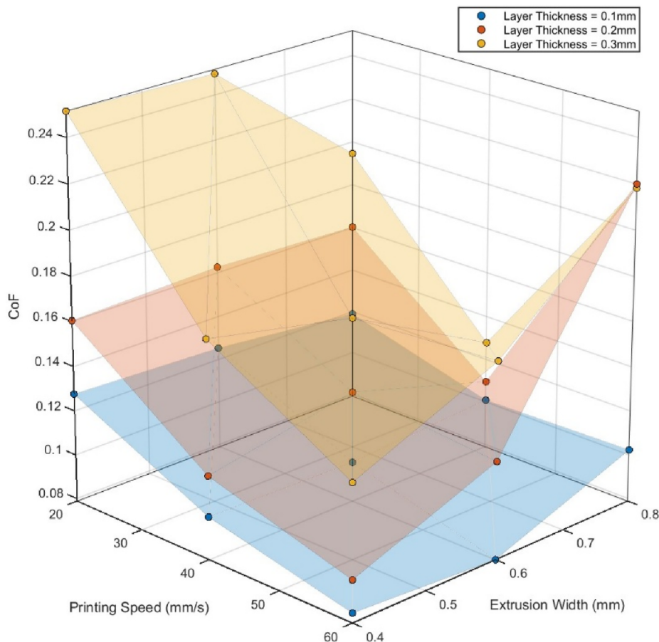
Fig. 7. Response surface of the CoF of the Plain surface as a function of printing speed and extrusion width at different layer thickness levels.
