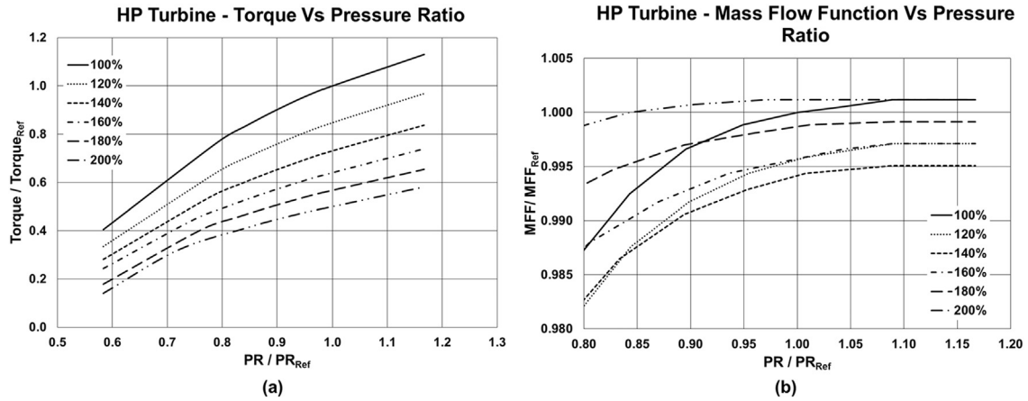
Fig. 5. HPT characteristic maps – (a) torque vs expansion ratio, (b) Mass flow function vs expansion ratio – for different non-dimensional speed functions.
