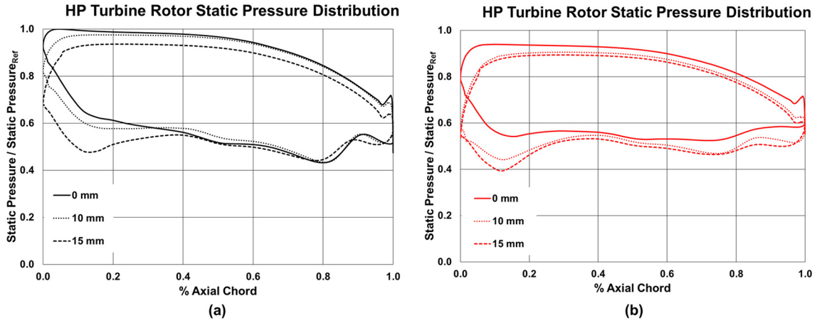
Fig. 11. Static pressure distribution in rotor tip aerofoil at different axial displacement locations. (a) No damage in tip seal fins. (b) Worn tip fins.
