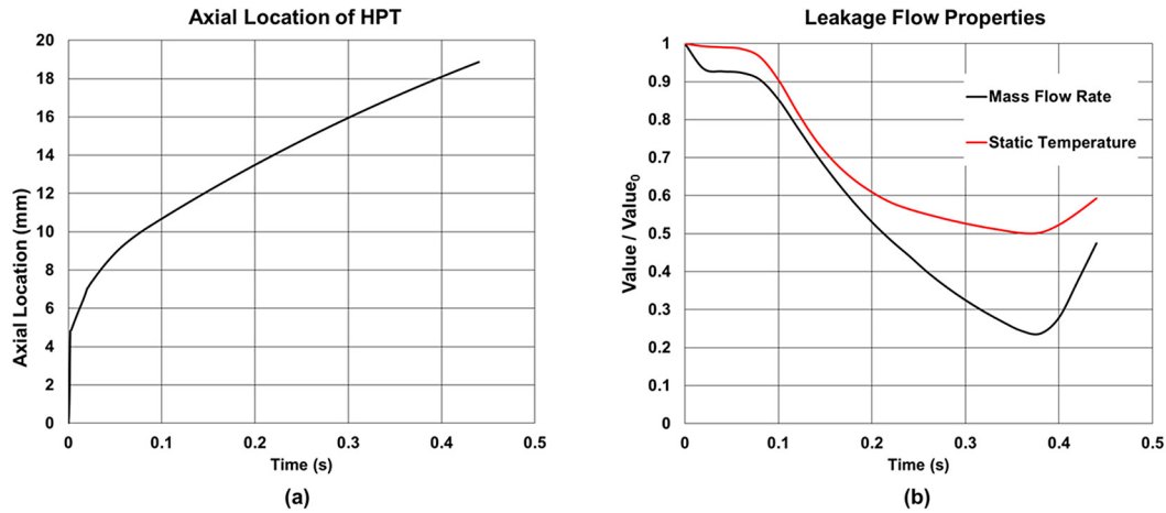
Fig. 1. (a) Axial location vs time from friction model. (b) Leakage flow rate and temperature vs time from secondary air system model.
