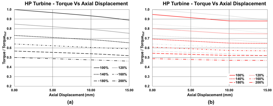
Fig. 8. HPT torque vs axial displacement at reference pressure ratio. (a) No damage in tip seal fins. (b) Worn tip fins.
