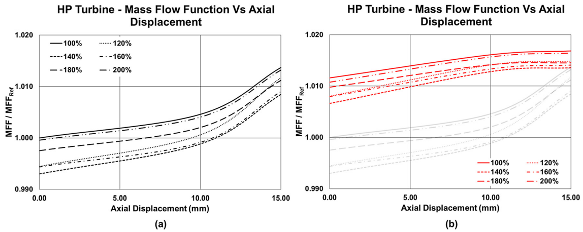
Fig. 9. HPT mass flow function vs axial displacement at reference pressure ratio. (a) No damage in tip seal fins. (b) Worn tip fins.
