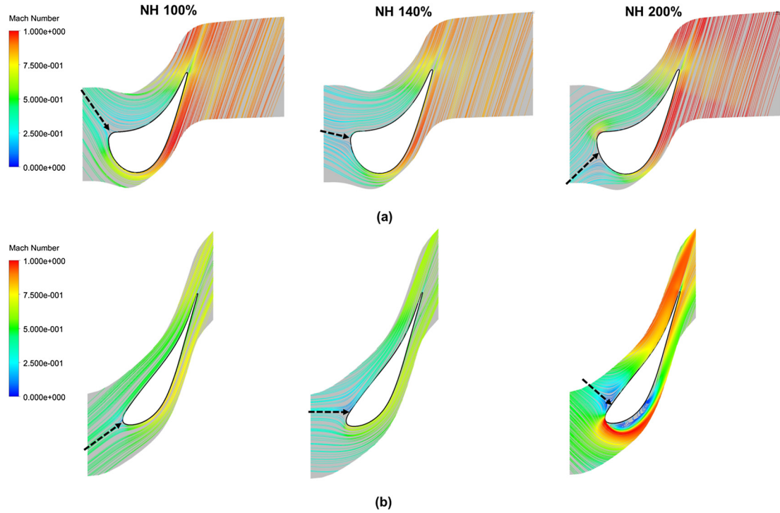
Fig. 7. Streamlines with arrows showing mean flow direction – (a) HP rotor mid plane relative Mach number, (b) IP stator mid plane absolute Mach number.
