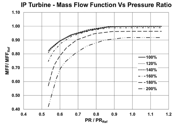
Fig. 6. IPT mass flow function vs expansion ratio – for different HPT non-dimensional speed functions.
