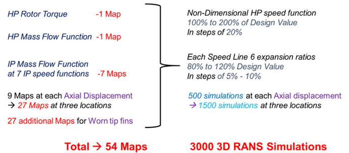
Fig. 2. Schematic showing extent of characterisation and flow simulations.
