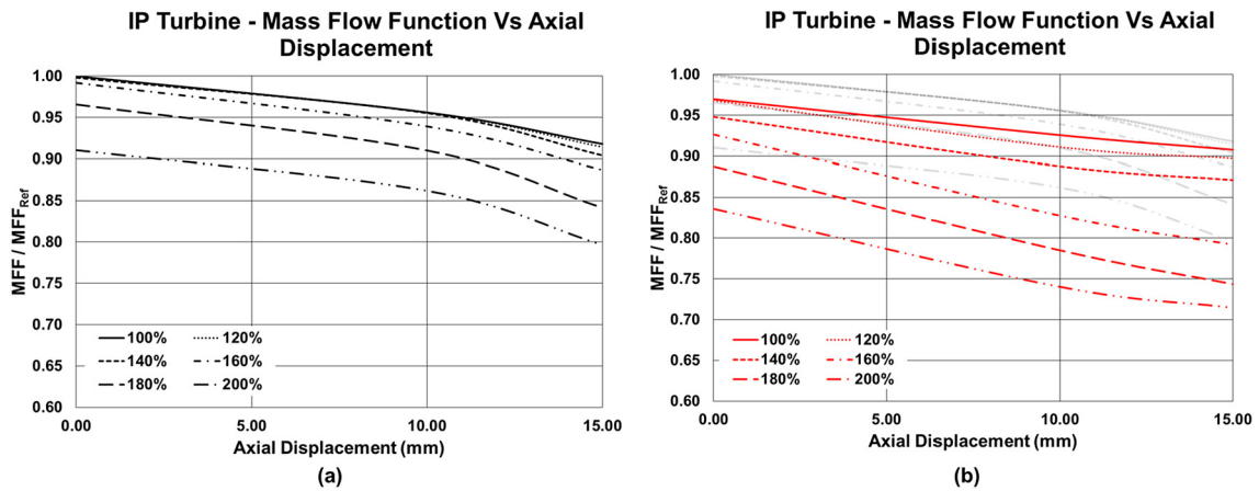
Fig. 10. IPT mass flow function vs axial displacement at reference IP pressure ratio. (a) No damage in tip seal fins. (b) Worn tip fins.
