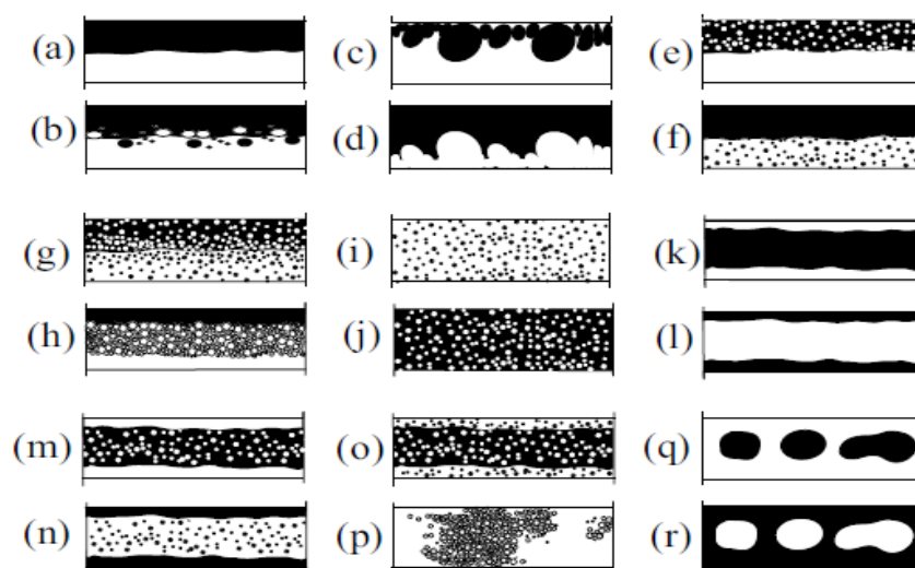
Figure 2. Typical flow patterns of oil-water in horizontal pipes [2]. Note: (a,b) Stratified flow of two separated layers (S, possibly with mixing at the interface, SM). (c,d) Stratified layers of a free-liquid and a dispersion of the other liquid (e.g., oil-in-water dispersion above a water layer, Do/w & w). (e,f) Stratified layers of a free liquid and a dispersion in the other liquid (e.g., oil and oil-in-water dispersion, Do/w & o; water and water-in-oil dispersion, Dw/o & w). (g,h) Layer of dispersions (e.g., water-in-oil dispersion above oil-in-water dispersion Dw/o & o/w, possibly with pure oil at the top and/or water at the bottom). (i,j) Fully dispersion or emulsion of one liquid in the other liquid (e.g., water-in-oil or oil-in-water dispersion or emulsion, Dw/o or Do/w). (k,l) Core-annular flow—a core of one liquid with the other liquid (e.g., a core of viscous oil and water in the annulus, ANw. Oil in the annulus, ANo). (m,n) Annular flow of a liquid with a dispersion in the core (water in the annulus DANw, oil in the annulus DANo). (o) Core-annular flow of two dispersions (CADw or CADo). (p) Intermittent flow (one liquid alternatively occupying the pipe as free liquid or as a dispersion, Io or Iw). (q,r) Larger elongated or spherical bubbles of one liquid in the other (SLo, Bo or SLw, Bw) [2].
