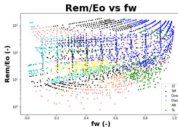
Figure 6. The ratio of mixture Reynold number to Eötvös number ( Re_m/Eo ) versus water fraction ( f_w ) for the gathered published experimental datasets. Note: data from [3,11,22,38,41,52,55–58]. Data points denoted with red squares, black rectangles, blue triangle_left, cyan triangle_down, yellow circle and green star represent stratified flow (ST), stratified mixed flow (SM), dispersed oil-in-water flow (Do/w), dispersed water-in-oil flow (Dw/o), annular flow (AN) and slug flow (SL), respectively.
