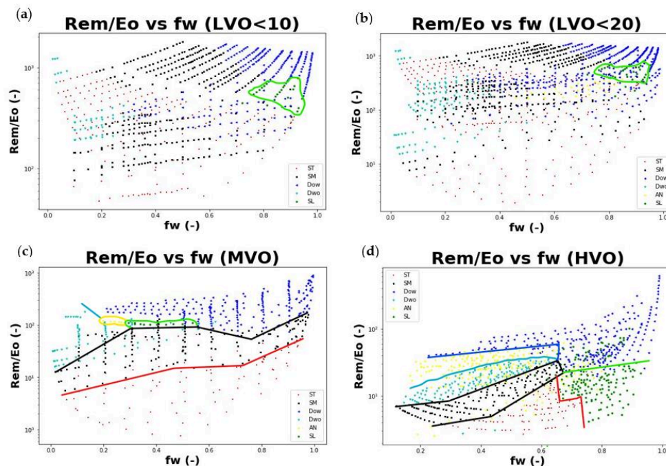
Figure 7. The ratio mixture Reynolds number to Eötvös number ( Re_m/Eo ) versus water fraction ( f_w ), (a) <10 mPa s (b) <20 mPa s (c) 20\text{--}100 mPa s, (d) >100 mPa s, for the gathered published experimental datasets. Note: data points denoted with red squares, black rectangles, blue triangle_left, cyan triangle_down, yellow circle and green star represent stratified flow (ST), stratified mixed flow (SM), dispersed oil-in-water flow (Do/w), dispersed water-in-oil flow (Dw/o), annular flow (AN) and slug flow (SL), respectively. Each boundary line denoted with red, black, blue, cyan, yellow and green encloses—partially or completely—stratified flow (ST), stratified mixed flow (SM), dispersed oil-in-water flow (Do/w), dispersed water-in-oil flow (Dw/o), annular flow (AN) and slug flow (SL), respectively.
