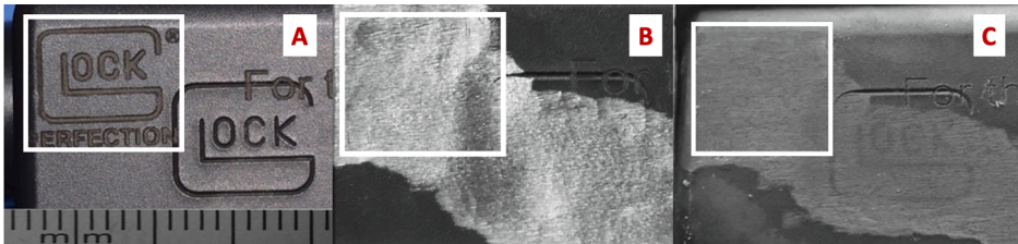
Fig. 7. The front left side of the pistol slide. (A) the marks before obliteration, (B) the marks after obliteration, and (C) the stamped “Glock” logo was recovered using Fry’s reagent, and the laser engraved logo was not recovered (boxes). Note; additional laser engraved text was not obliterated and can be seen overlapping the Glock logo.
