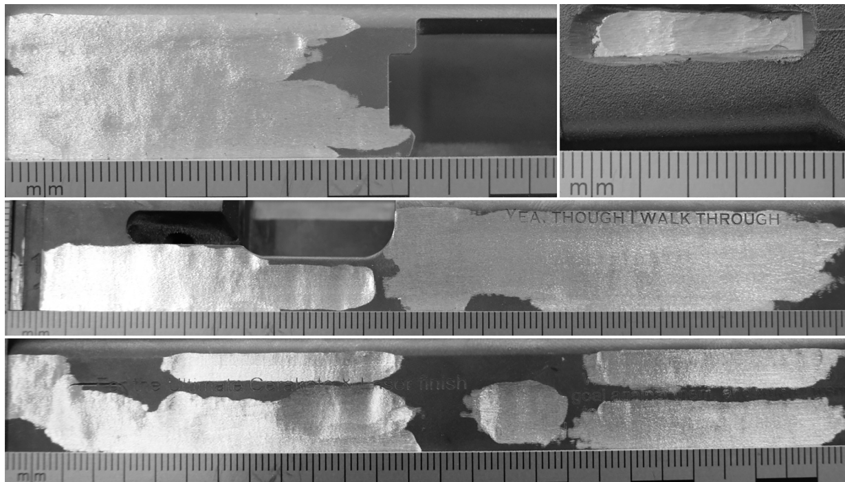
Fig. 4. Each side of the pistol slide (top, middle) and the backface of a top cover (bottom) after the marks were removed with a Dremel®.
