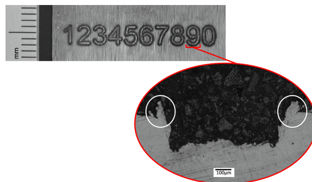
Fig. 1. One laser engraved serial number on a steel plate (left) and a cross section of the highlighted character (×50 magnification), showing the depth of the laser engraving (230 µm) (right). The lipping of the metal is circled.
