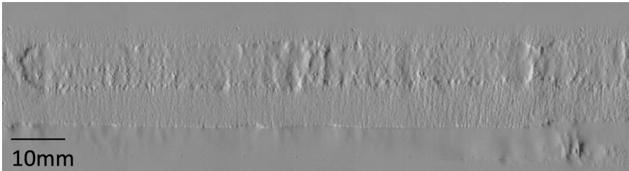
Fig. 8. The electromagnetic recovery image showing the microstructure of the AK-pattern rifle top cover, where the laser engraved marks were removed by hand using a Dremel® rotary tool.
