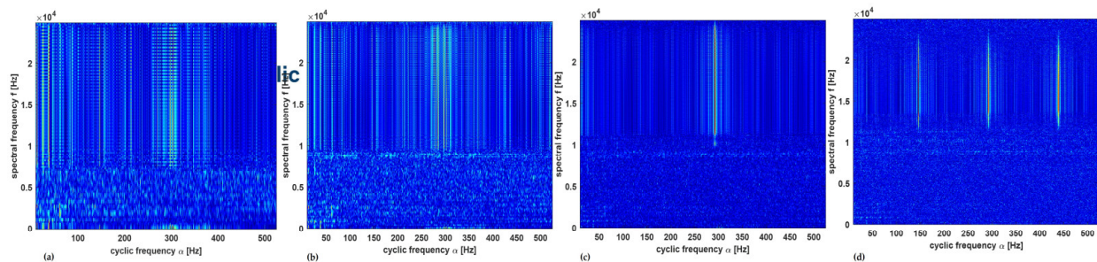
Figure 7. Cyclic spectral coherence maps for healthy shaft at window size: (a) 128, (b) 256, (c) 512, and (d) 1024.
