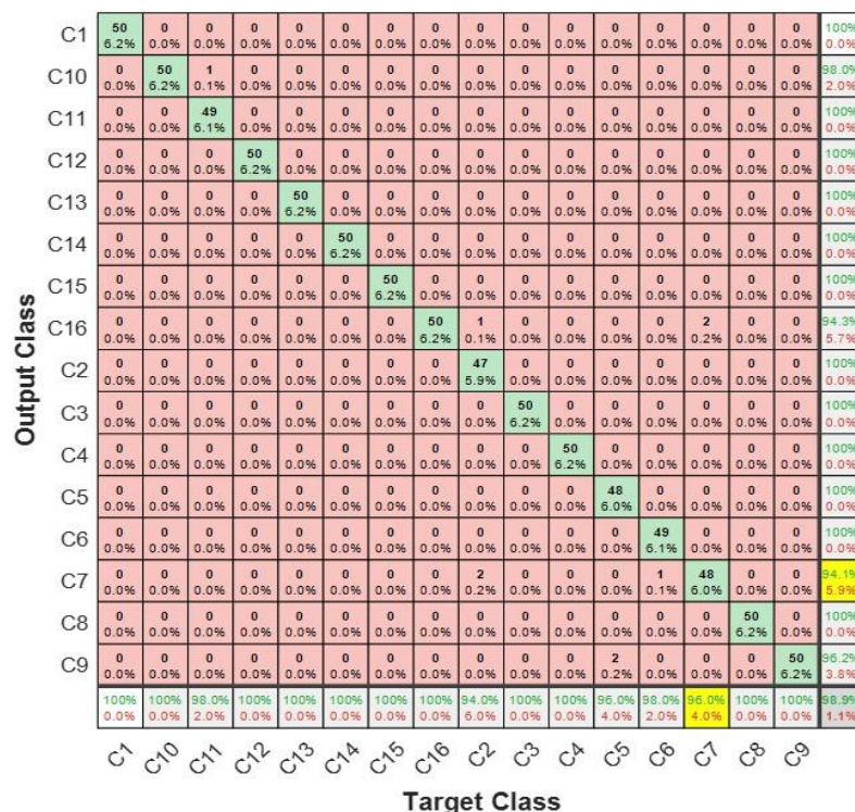
Figure 13. Confusion matrix for the proposed ensemble model implementation.
