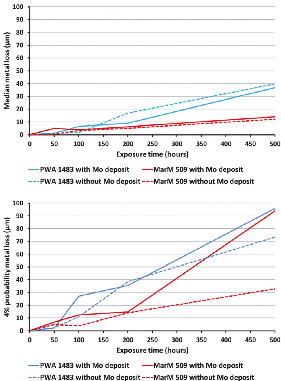
Figure 4. Median (top) and 4% (bottom) probability of metal loss exceedance plots. Exposure carried out at 700 °C in an air atmosphere with 300 ppm SO 2 . The deposit flux was 1.5 μg/cm 2 /h of 80/20 (Na/K) 2 SO 4 either modified with 1.5 μg/cm 2 /h of molybdenum or unmodified [8].
