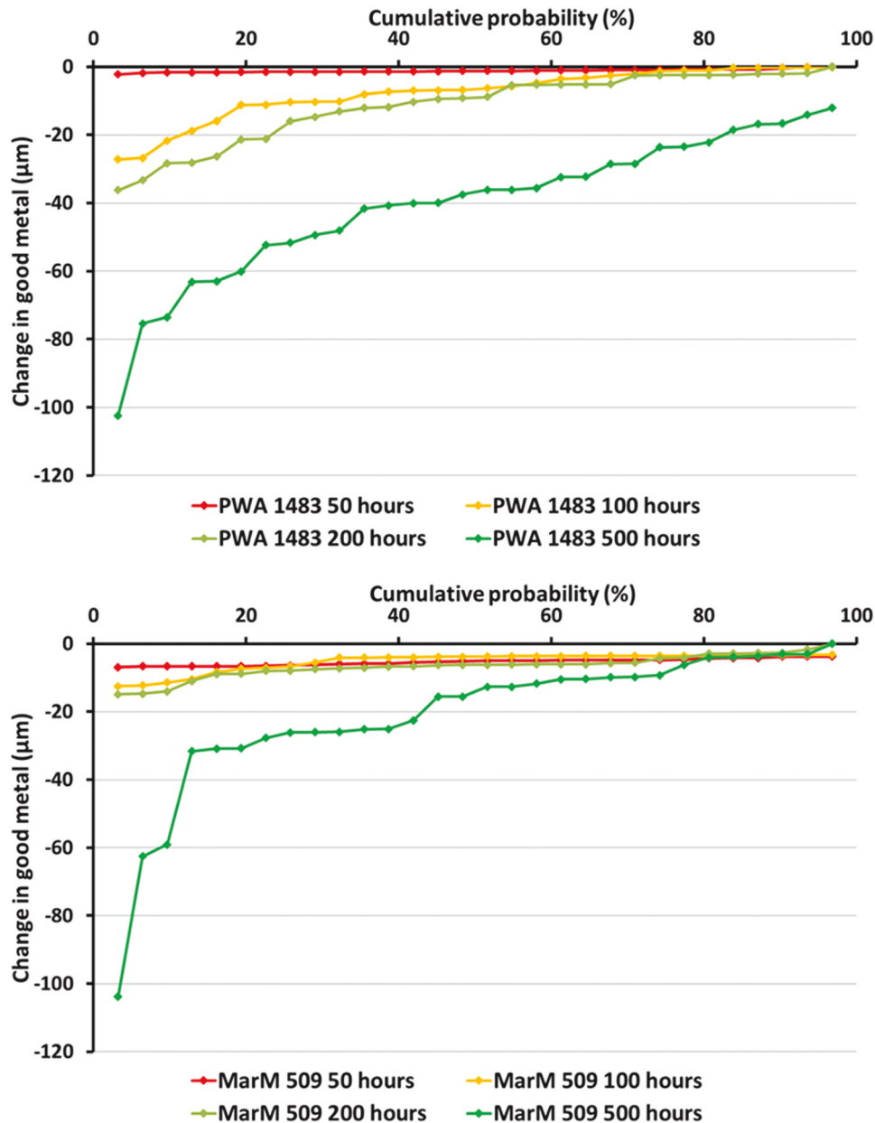
Figure 3. Cumulative probability of change in good metal plots for PWA 1483 (top) and MarM 509 (bottom). Exposure carried out at 700 °C in an air atmosphere with 300 ppm \text{SO}_2 . The deposit flux was 1.5 \mu\text{g}/\text{cm}^2/\text{h} of 80/20 (\text{Na/K})_2\text{SO}_4 modified with additions of 1.5 \mu\text{g}/\text{cm}^2/\text{h} of Mo.
