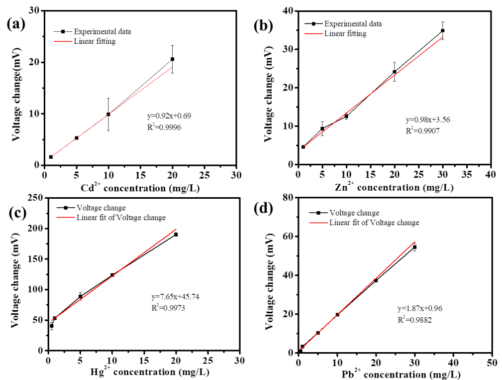
Figure 4. The calibration curves for \text{Cd}^{2+} (a), \text{Zn}^{2+} (b), \text{Hg}^{2+} (c), or \text{Pb}^{2+} (d) as detected by the developed SMFC-based sensing system.
