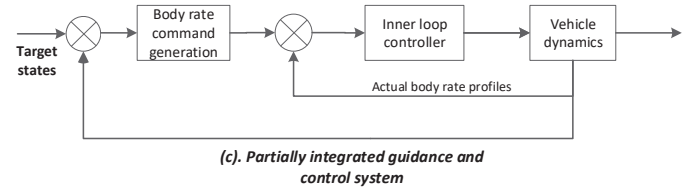
Figure 2: Typical space/aerospace vehicle guidance and control systems
