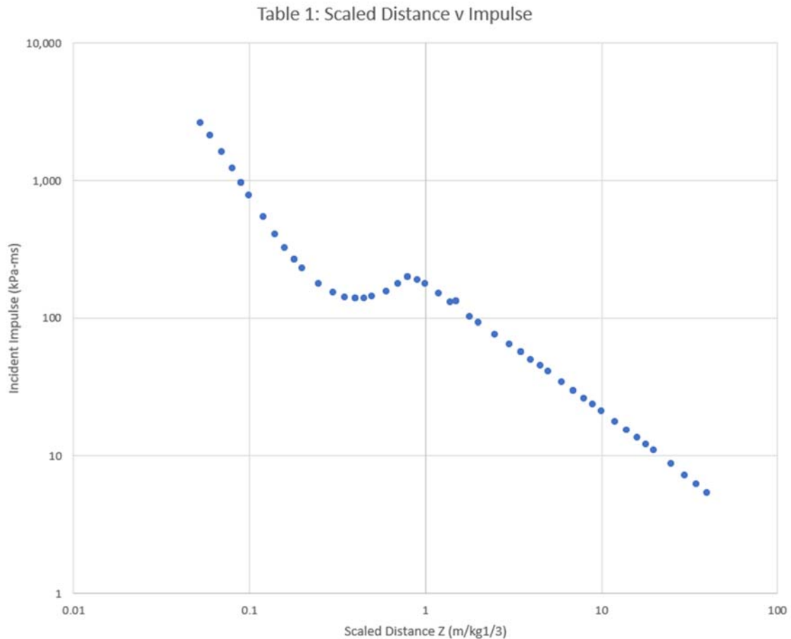
Fig. 2. Kingery & Bulmash data for 1kg Spherical TNT charge [9, Tbl. 1] showing a major discontinuity that appears common with impulse
