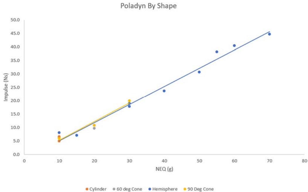
Fig. 5. Comparison of results with different charge shapes Poladyn show that the charge shape has relatively little effect on the impulse measured
