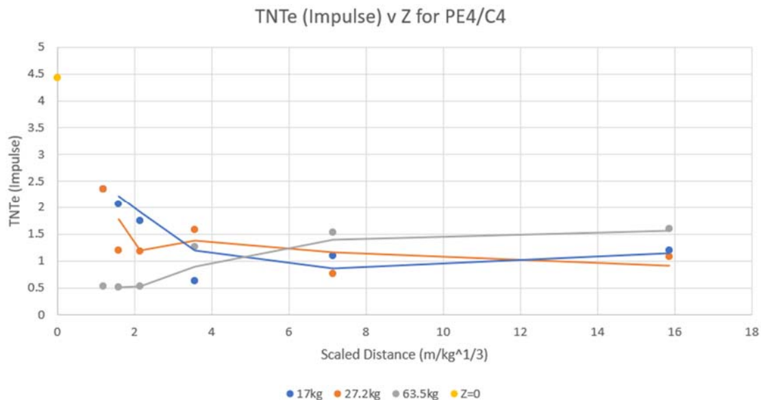
Fig. 7. Plotting McIntyre's TNTe (Impulse) for C4 and this trial's comparable figure, one can see that the two smaller NEQ charges from McIntyre show a sudden increase as Z reduces. Extrapolating back to the Y axis, they would meet the axis close to the Z=0 figure [13, Tbls. 2–4].
