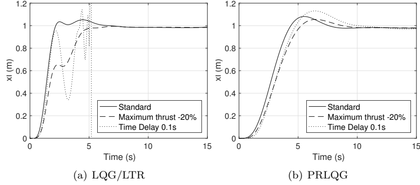
Figure 13: Effect of system parameters in 4-UAV transportation system
