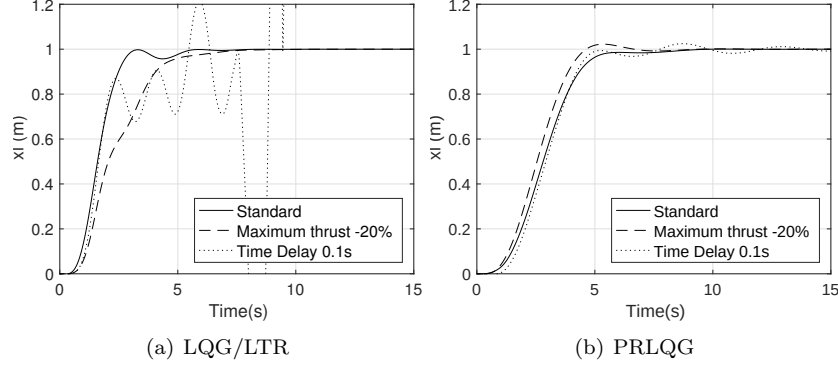
Figure 11: Effect of system parameters in 1-UAV transportation system
