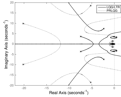
Figure 8: Root locus of PRLQG
