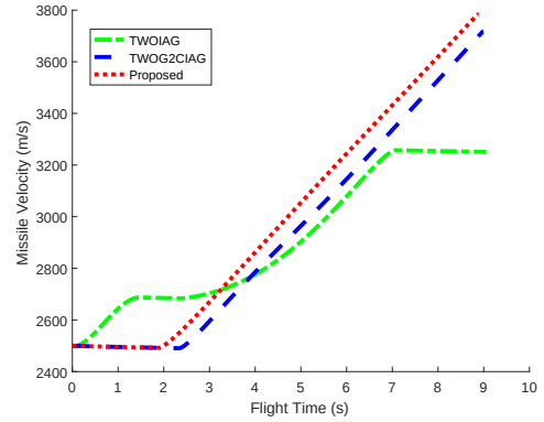
Fig. 11. Missile velocity profile.
