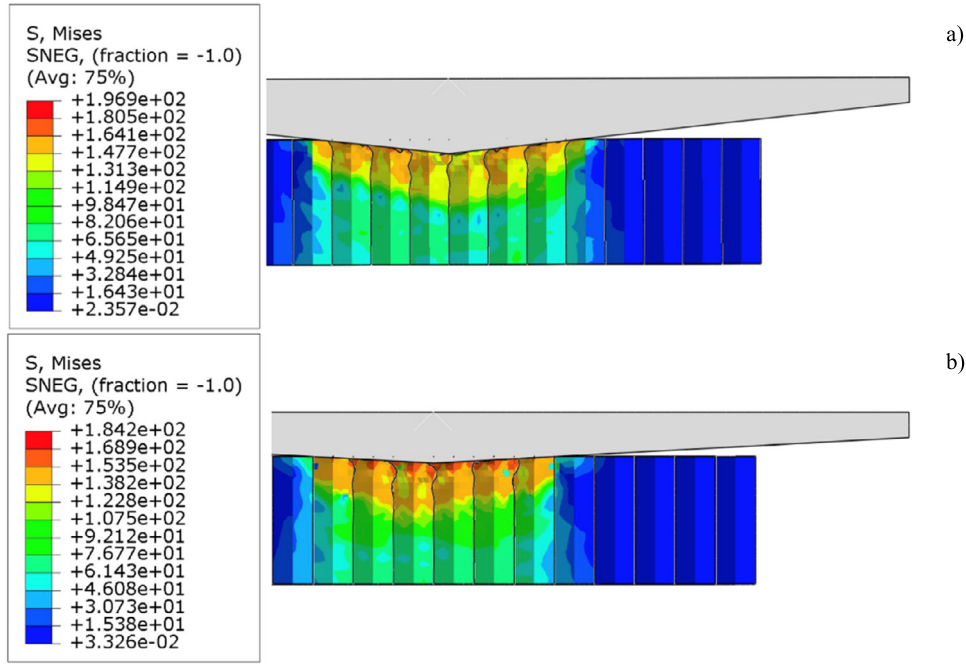
Fig. 5. High fidelity stress distribution in the core under the contact patch for: a) \psi = 86.947^\circ and b) \psi = 83.912^\circ .
