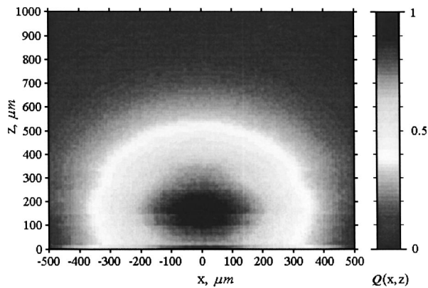
Fig. 5 Two-dimensional distributions of the spatial depth sensitivity Q(x, z) . The optical parameters of skin layers were chosen for 488 nm (Table 1). The fraction of fluorescence that is sensitive to sensor and topical dermal layers is close to one another. The diameter and numerical aperture of the detector are equal to 1000 \mu\text{m} and 0.63; acceptance angle \theta_d = \sin^{-1}(NA/n_0) is 40^\circ with NA the numerical aperture.
