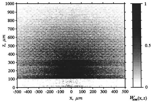
Fig. 4 Spatial distribution W_{em}(x, z) of the fluorescence excitation of the tattoo sensor layer embedded in the epidermis and autofluorescence excitation in human skin. Optical parameters of the model were chosen for 488 nm (see Table 1). The diameters of collagen bundles were chosen as 3, 6, 20, and 30 \mu\text{m} in papillary dermis, upper blood net dermis, dermis, and deep blood net dermis, respectively. The diameter of the source is equal to 200 \mu\text{m} . The incident beam has a uniform geometry profile.
