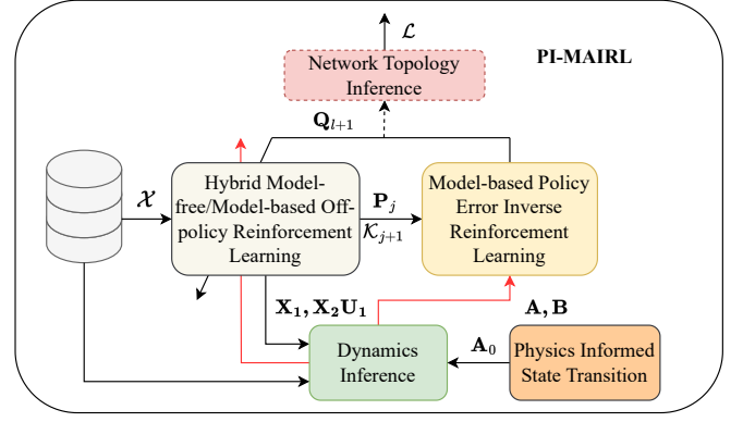
Fig. 2. PI-MAIRL high-level diagram
