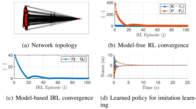
Fig. 10. Results for the 50 drones case
