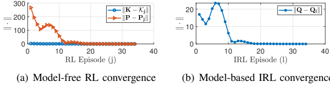
Fig. 9. Convergence results for the five drones case
