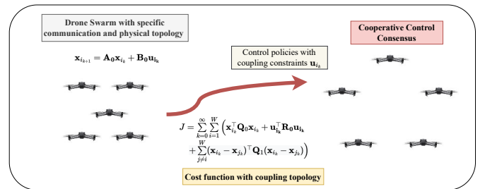
Fig. 1. Drone swarm modelling for cooperative control/consensus
