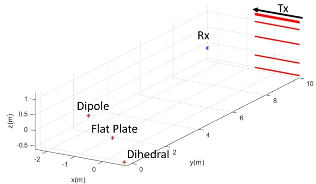
FIGURE 2 | Sparse bistatic SAR simulation geometry. The transmitter aperture (red) is labelled as Tx and receiver position is as labelled Rx. The flat plate, dihedral and dipole scatterers are labelled in the scene.
