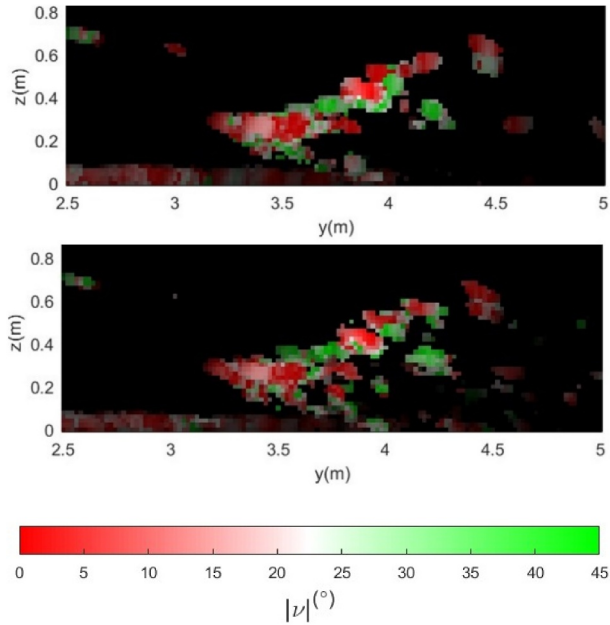
FIGURE 17 | PolSSARVI point-cloud MIPs in the y-z plane, showing a side view of the tank rendering. Colour indicates the skip angle, with brightness determined by the polarimetric span in dB, with a 50-dB dynamic range. The renderings were formed at SIS sampling (top) and at 52% ARF-SIS (bottom).
