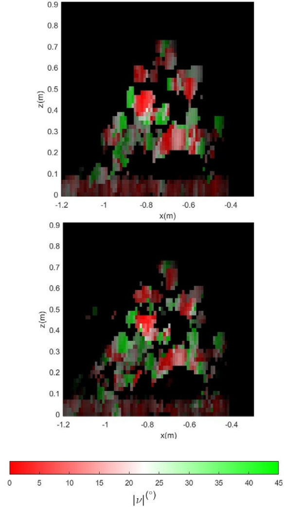
FIGURE 15 | PolSSARVI point-cloud MIPs in the x-z plane, showing a front view of the tank rendering. Colour indicates the skip angle, with brightness determined by the polarimetric span in dB, with a 50-dB dynamic range. The renderings were formed at SIS sampling (top) and at 52% ARF-SIS (bottom).
