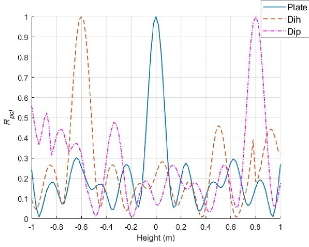
FIGURE 3 | Summed interferometric response R_{\text{pol}} along vertical iso-range arcs through the location of the flat plate, dihedral and dipole scatterer. These are labelled as Plate, Dih and Dip, respectively.
