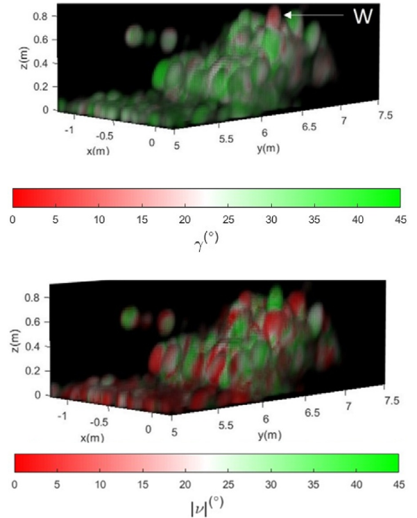
FIGURE 8 | Multistatic 3D BPA SAR images of the model vehicle, formed with the full transmitter aperture presented in Figure 6. Polarimetric span-intensity in dB provides the brightness in these images, and colour is attributed to polarimetric parameter angles. The polarisability angle is shown (top) together with the skip angle (bottom). ‘W’, in the top rendering, denotes the position of the wire, which is seen to have a high polarisability value.
