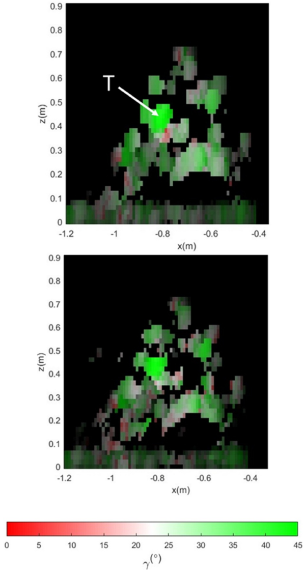
FIGURE 14 | PolSSARVI point-cloud MIPs in the x-z plane, showing a front view of the tank rendering. Colour indicates the polarisability angle, with brightness determined by the polarimetric span in dB, with a 50-dB dynamic range. The renderings were formed at SIS sampling (top) and at 52% ARF-SIS (bottom). The turret is labelled as ‘T’.
