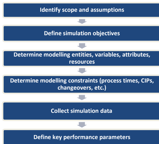
Fig. 3. Discrete Event Simulation Methodology
