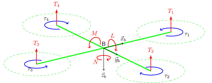
Fig. 1. Thrust, Forces and Moments on Quadrotor
