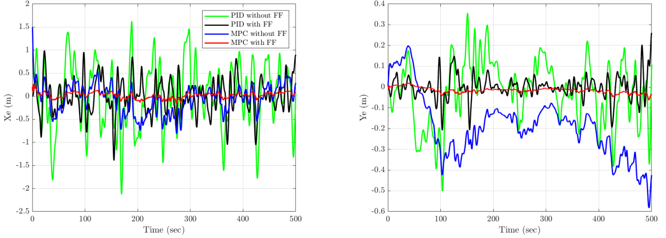
Fig. 9. Comparison of MPC with PID Control Law
