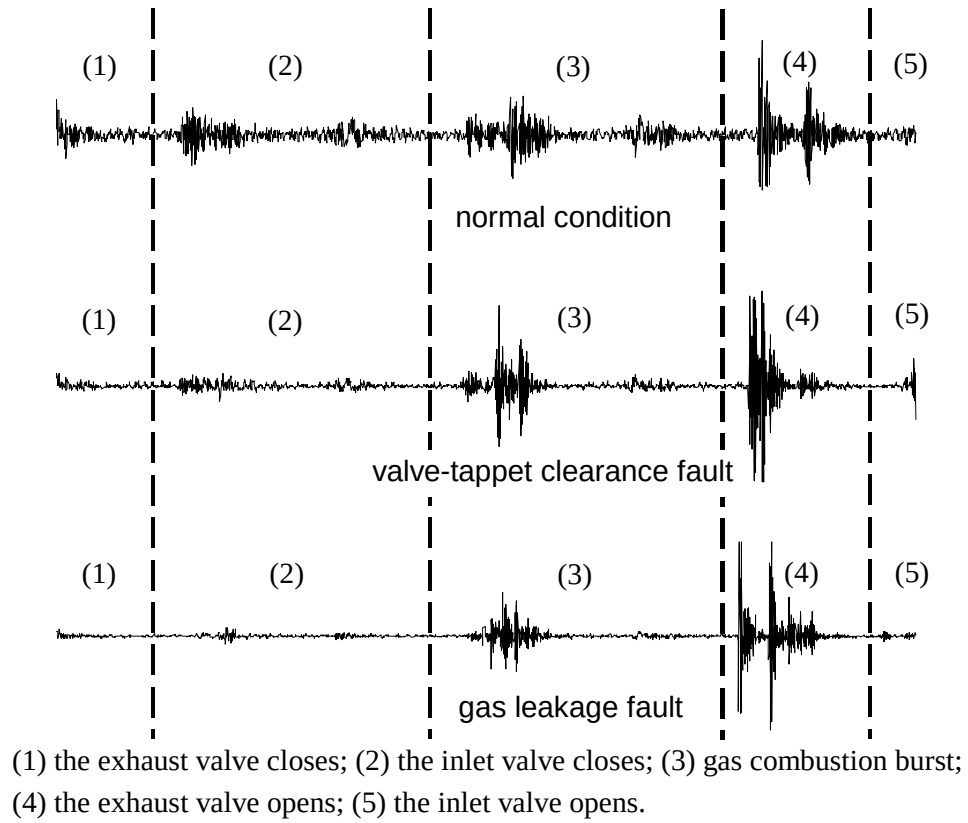
Fig.1 Vibration signal collected from the exhaust valve of the engine
