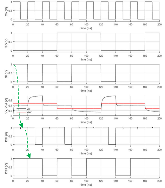
Fig. 10. Simulation results of the various signals in the proposed SBS Transceiver Circuit in Fig. 9. (Vertical scale normalized to V_{dd} ).
