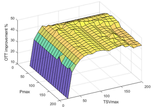
Fig. 15: % improvement in OTT of SIC 3 with varying Pins and TSV limits
