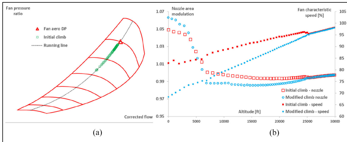
Figure 9. (a) Fan characteristic speed, (b) Variable area nozzle modulation.
