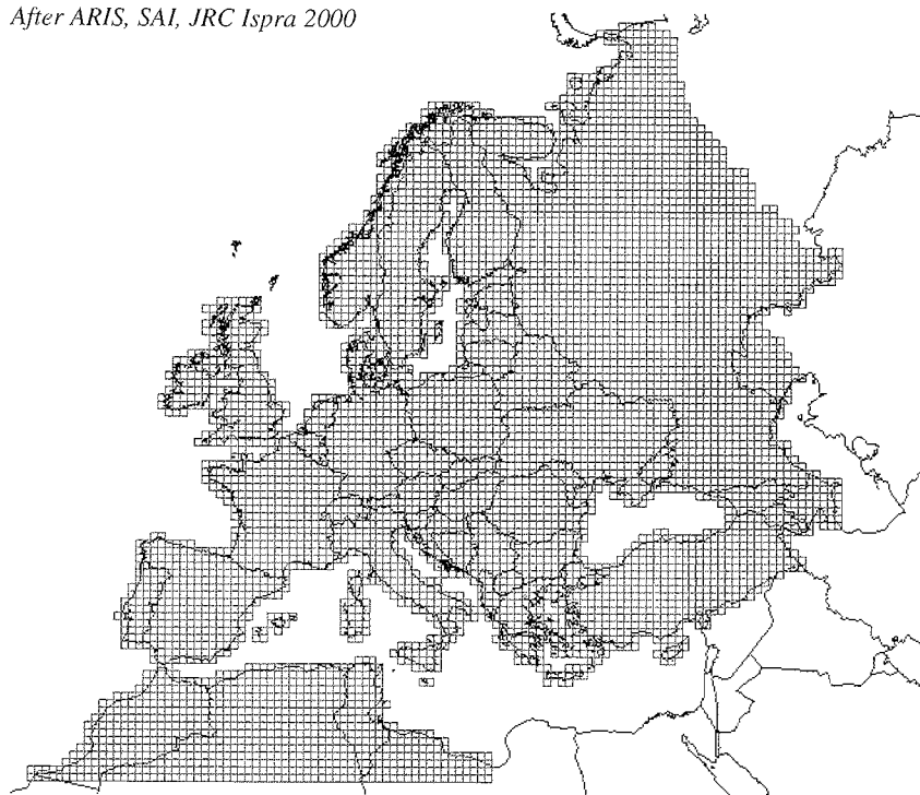
Figure 6. The 50 km \times 50 km grid of the MARS meteorological database.
