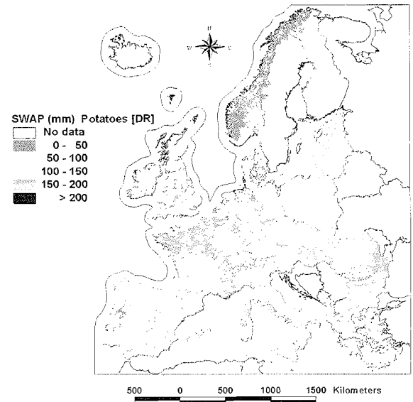
Figure 5. Soil water available to plants, SWAP (mm) for a short rooting crop e.g. potatoes.
