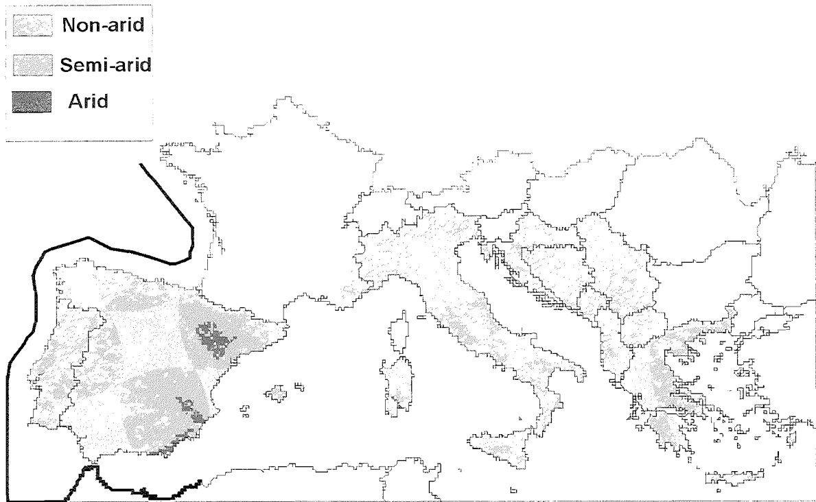
Figure 3. The approximate extent in Europe of soils inferred as arid from soil classification.
