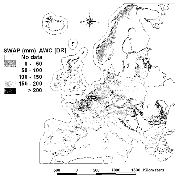
Figure 4. Soil water available to plants, SWAP (mm) to 1 m depth or to a rooting restriction.
