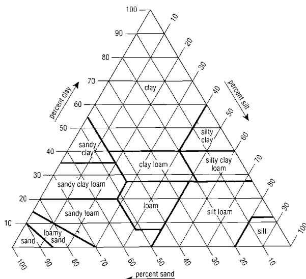
Figure 1. Soil texture classes (Schoeneberger et al. 1998).
