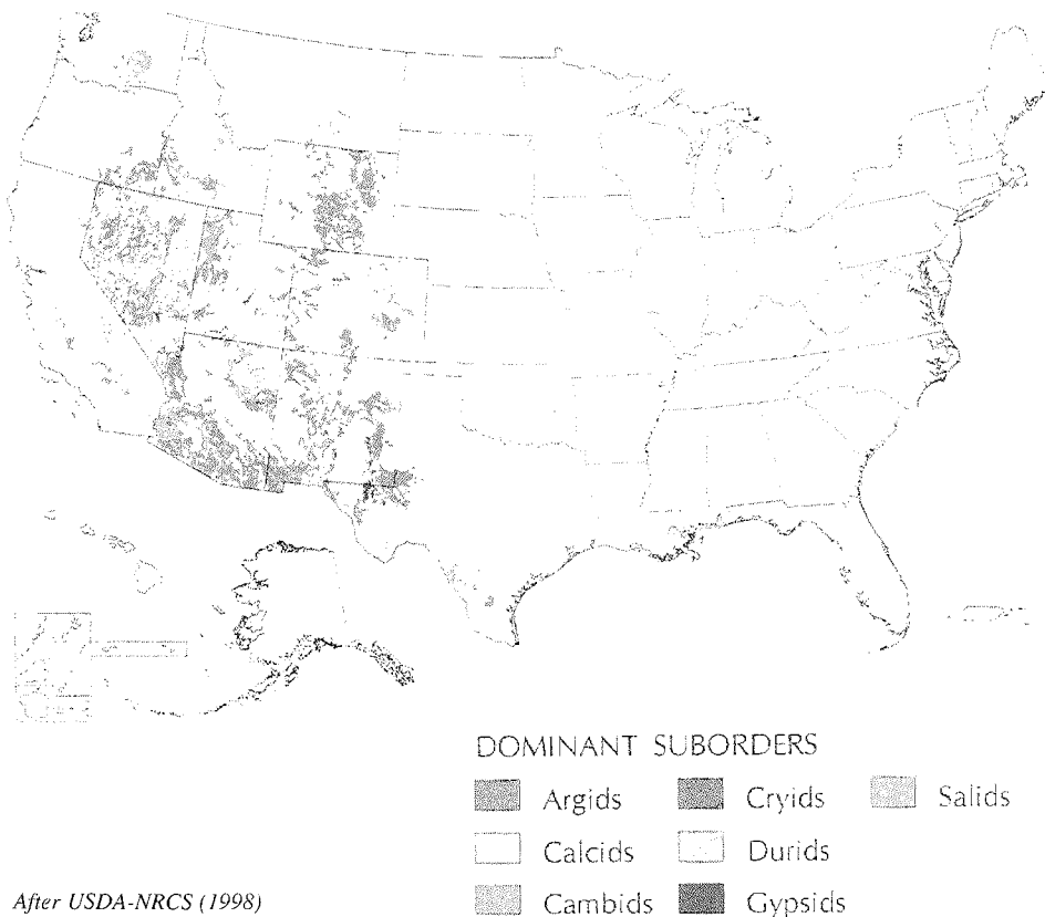
Figure 2. The approximate extent in USA of soils classified as arid according to soil taxonomy.
