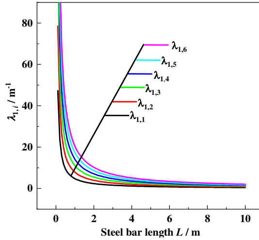
Fig. 4 The relationship between \lambda_{1,i} and the steel bar length.
