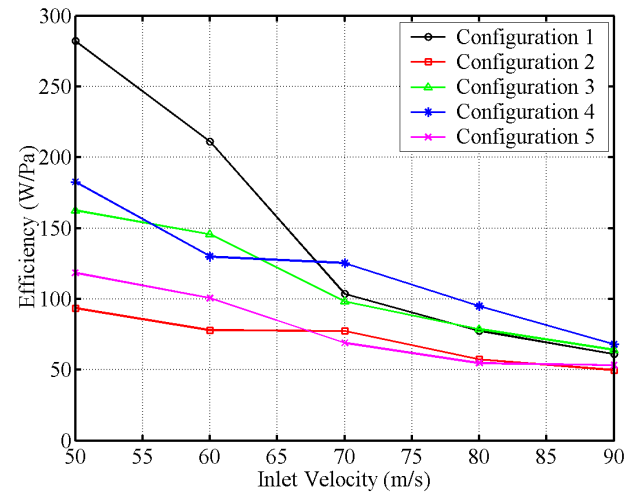
Figure 8: Efficiency of the investigated heat exchanger configurations.
