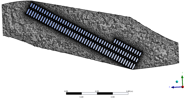
Figure 2: Computational mesh of the heat exchanger Configuration 3 placed in the sidepod with approximately 25 million elements.
