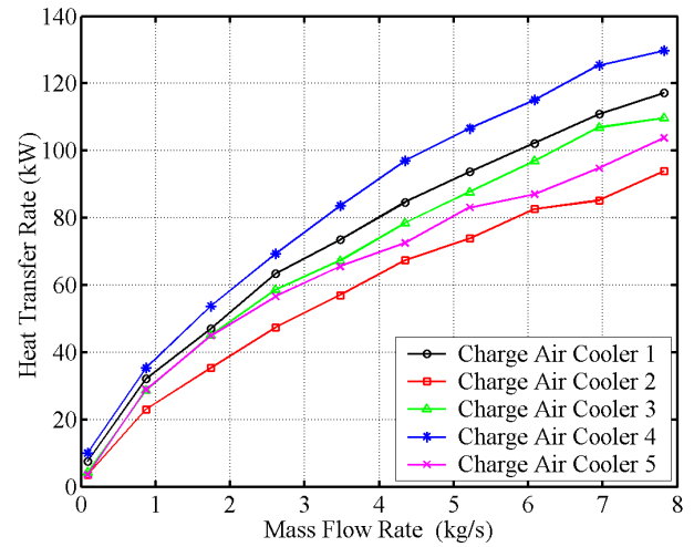
Figure 6: Charge air cooler heat transfer rate (kW) versus mass flow rate (kg/s) correlation curves.
