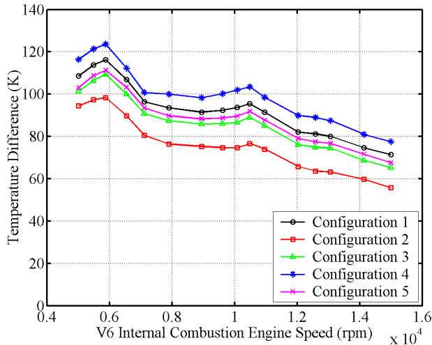
Figure 10: Temperature difference ( K ) versus V6 internal combustion engine speed ( rpm ) correlation curves for each configuration.
