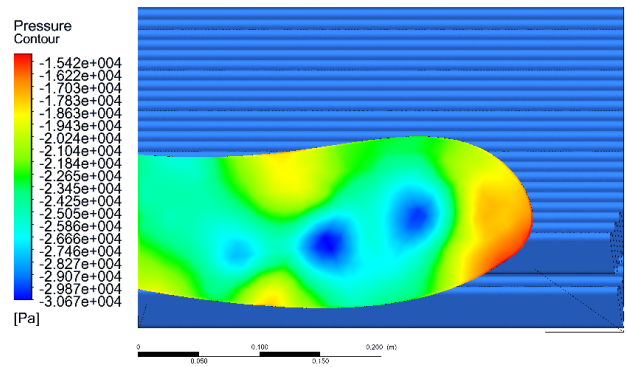
Figure 12: Outlet face pressure distribution relative to inlet face.
