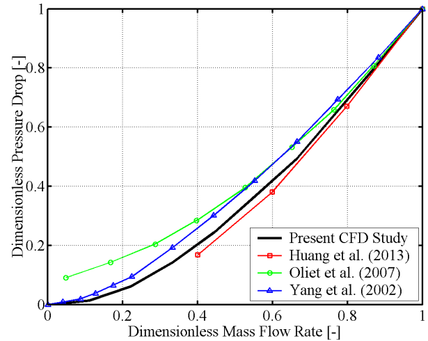
Figure 3: Dimensionless pressure drop [-] versus dimensionless mass flow rate [-] curve of the heat exchanger Configuration 2 compared to other studies.
