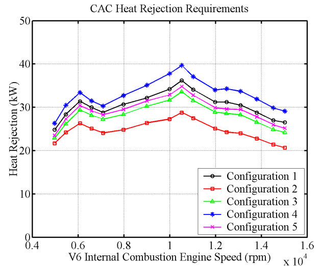
Figure 9: Charge air cooler (CAC) heat rejection (kW) versus V6 internal combustion engine speed (rpm) correlation curves for each configuration.
