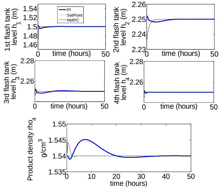
Fig. 10. NMPC & PI Control performance for a step increase in feed temperature from 60 to 66^\circ\text{C} .
