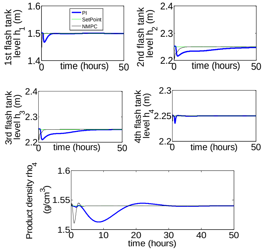
Fig. 9. NMPC & PI Control performance for a step decrease in feed density from 1.310 to 1.245 \text{ g/cm}^3
