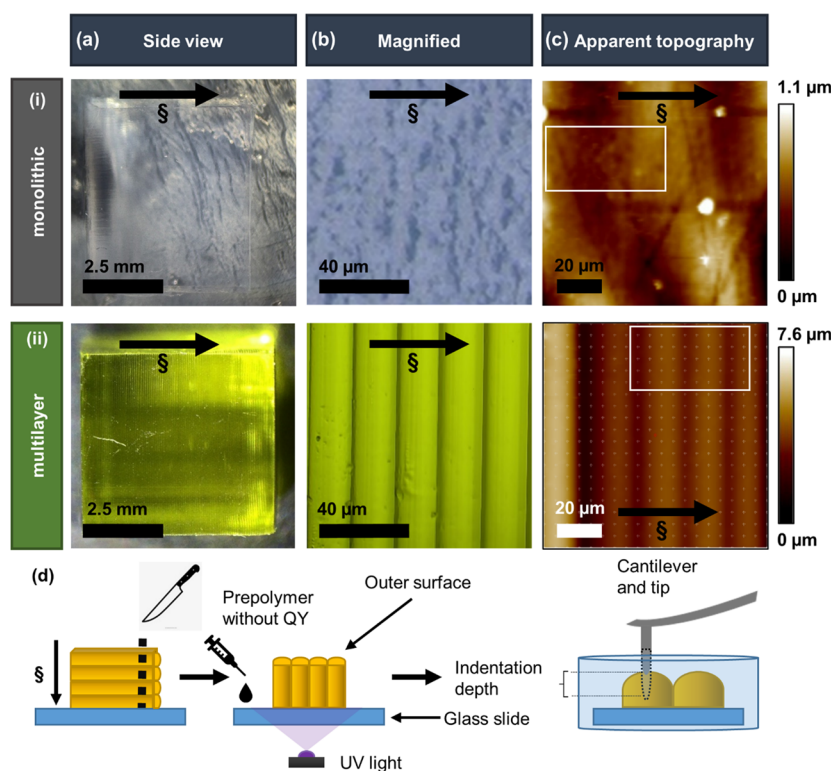
Figure 1. (a) Side view, (b) magnified optical microscopy images, and (c) apparent topography recorded with AFM peak force tapping mode (ramp) on the outer surface of (i) monolithic and (ii) multilayer PEGDA samples. (d) Schematic of sample preparation for the outer surface section of the multilayer sample. The white boxes were analyzed further for modulus measurements in Figure 2. Direction of projected light (§) is from top to bottom of the structure.
