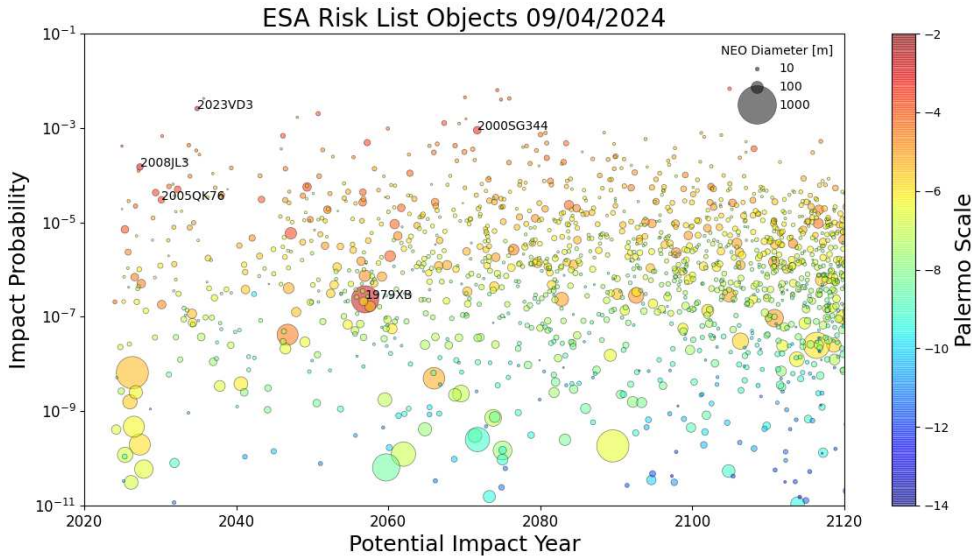
Figure 5. All the objects in the Risk List on 9 April 2024, represented in the plane (Potential Impact Year, Impact Probability). Only the VI with the largest PS is represented. The colour code represents the value of the PS, while the size of the marker is proportional to the diameter of the object.
