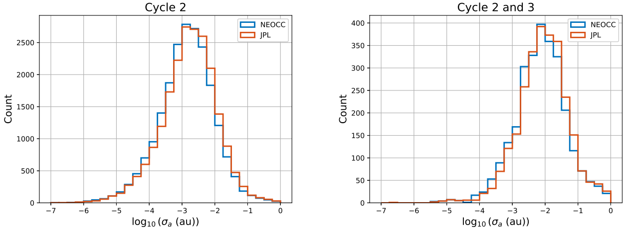
Figure 12. Distributions of uncertainty \sigma_a in the semi-major axis of NEAs which needed the execution of Cycle 2 of the global algorithm of differential corrections (left panel), and which needed the execution of Cycle 2 and 3 (right panel).
