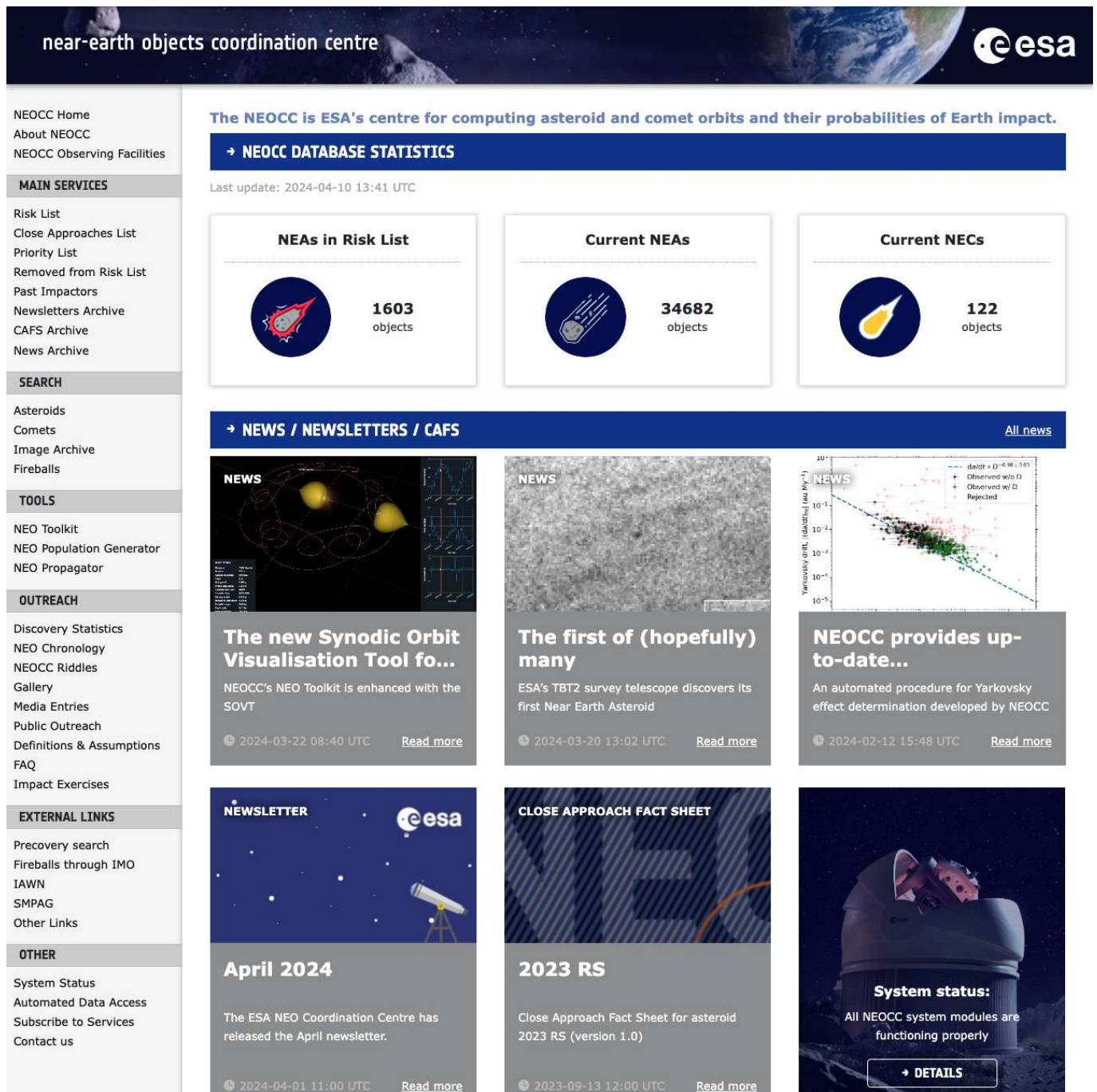
Figure 4. Main page of the NEOCC web portal. Statistics of the orbital database are graphically represented at the top of the web page, while recent news, newsletters, CAFS, and the System Status are shown right below. All the services provided by the NEOCC are accessible through the menu on the left.
