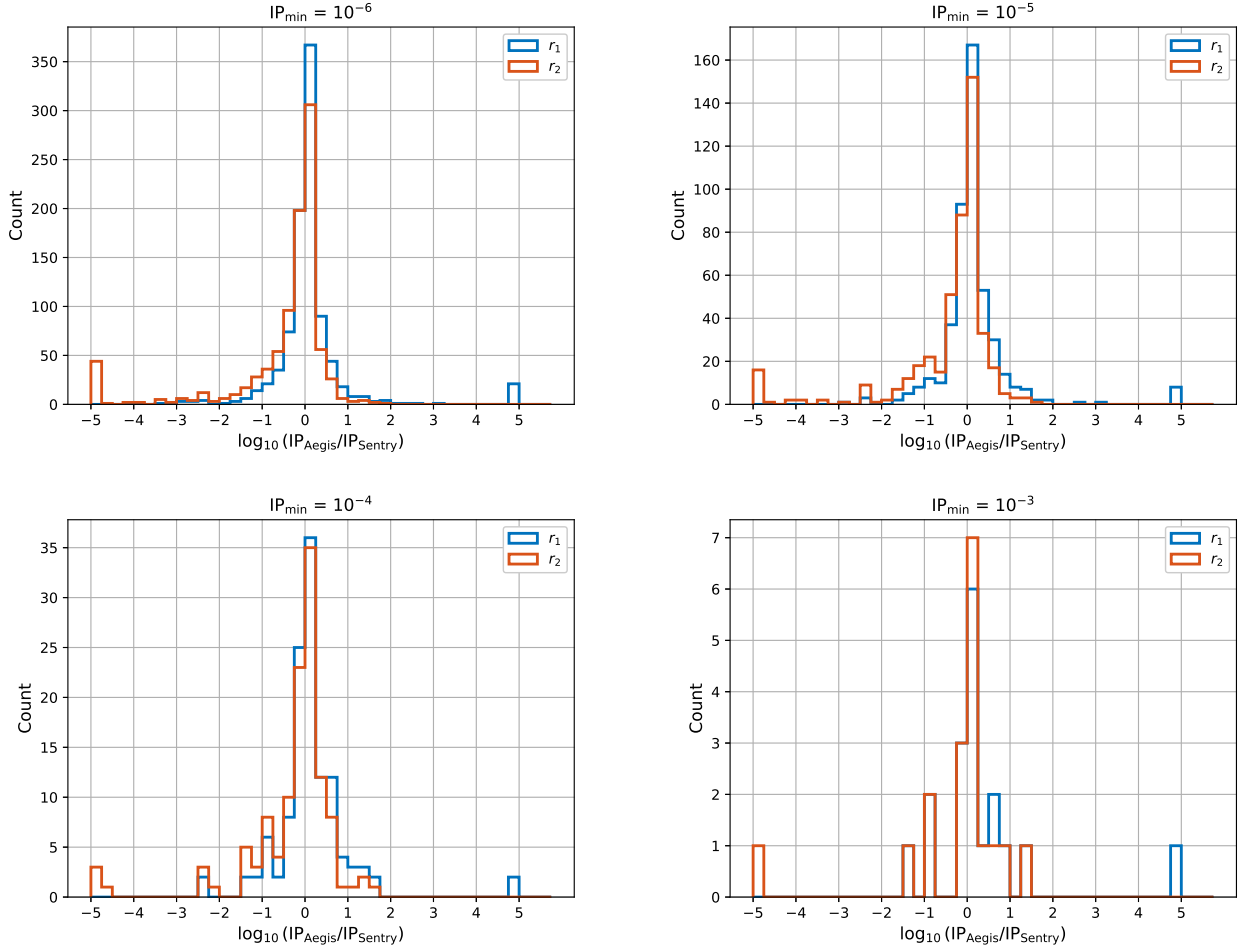
Figure 16. Distributions of the IP ratios r_1 (blue histogram) and r_2 (red histogram), obtained with equi-spaced bins with width equals to 0.25.
