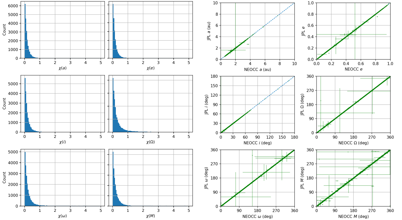
Figure 14. Same as Fig. 13, but obtained by taking into account only unnumbered NEAs. High resolution versions of these figures are provided as supplementary electronic material.
