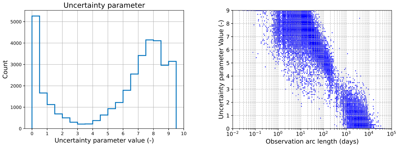
Figure 10. Left panel: distribution of the uncertainty parameter U for all the NEAs. Right panel: distribution uncertainty parameter U vs. arc length of all the NEAs.
