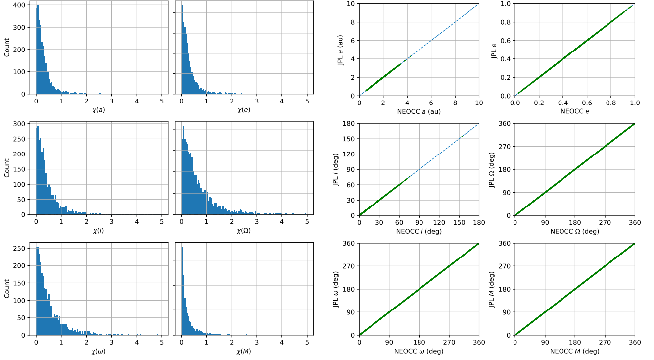
Figure 13. Distributions of \chi(y) for each Keplerian element y , obtained from the comparison of the orbits computed by the NEOCC and the JPL (first and second column), and distribution of y_{\text{NEOCC}} vs. y_{\text{JPL}} (third and fourth columns). The results shown here are obtained by taking into account only numbered NEAs. High resolution versions of these figures are provided as supplementary electronic material.
