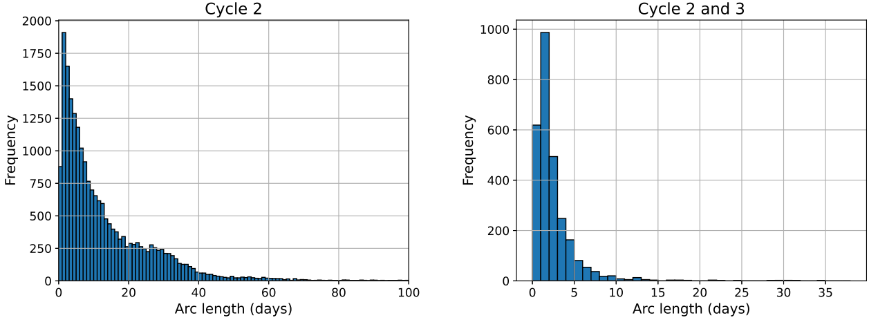
Figure 11. Distributions of the arc length of NEAs which needed the execution of Cycle 2 of the global algorithm of differential corrections (left panel), and which needed the execution of Cycle 2 and 3 (right panel).
