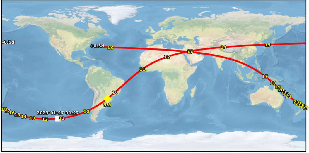
Figure 9. Ground track of asteroid 2023 BU (red curve) during its close approach with Earth on 27 January 2023. The white square corresponds to the epoch of minimum distance, while the yellow square represents the position at the brightness peak. Yellow numbers along the ground track denote the visual magnitude of the NEA as seen from the corresponding point on the Earth.
