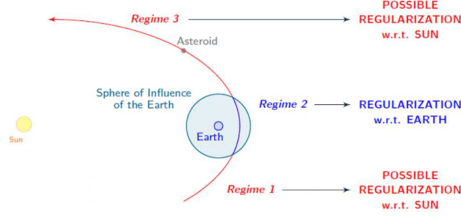
Figure 2. Example of an asteroid having a close approach with the Earth, where the global propagation is split into three different local propagations with different dynamical regimes.
