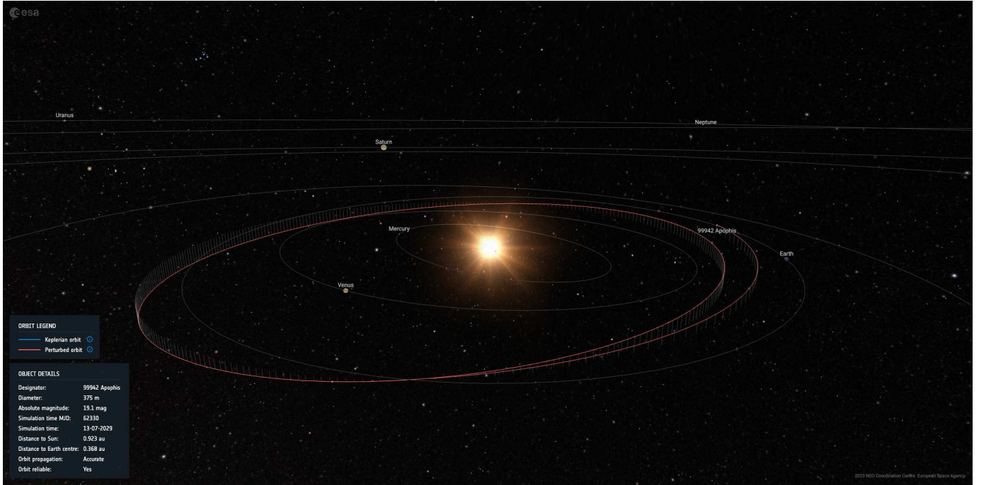
Figure 7. Perturbed orbit of asteroid (99942) Apophis around the epoch 13 July 2029, a few months after the Earth close approach, shown in the OVT.
