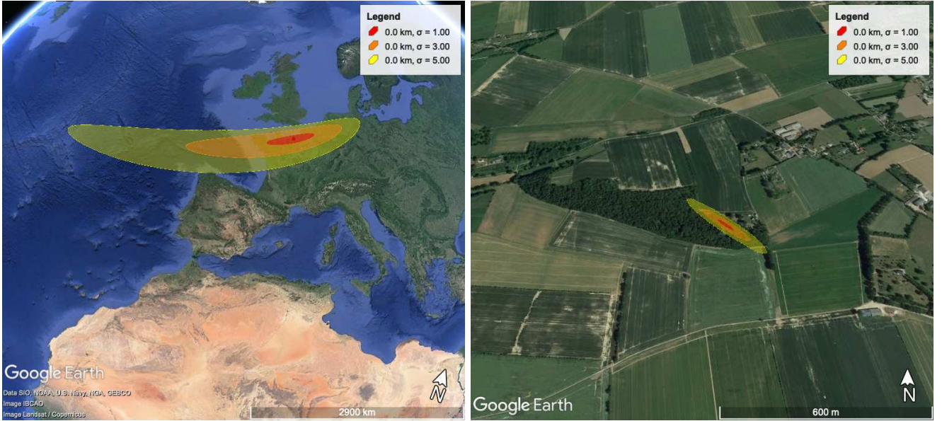
Figure 3. Impact corridor of 2023 CX 1 on the ground, a small NEA which impacted Earth 2023-02-13. The left panel shows the results obtained with just the first 7 observations, while the right panel the results obtained with all the observations available. The red, orange, and yellow areas represent the impact area at 1- \sigma , 3- \sigma , and 5- \sigma level, respectively. The last part of the numerical integration has been performed without taking into account the atmospheric drag.
