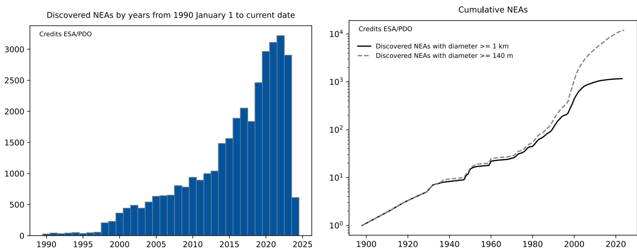
Figure 1. Left panel: distribution of discovered NEOs from 1990 to current date, binned by year. Right panel: cumulative distribution of discovered NEOs larger than 1 km (black thick curve), and of NEOs larger than 140 m (grey dashed curve). In the right panel plot, the diameter is obtained by converting the absolute magnitude H into diameter D with the formula D = 1329 \text{ km} / \sqrt{p_V} \times 10^{-H/5} (Bowell et al., 1989; Pravec and Harris, 2007), where the albedo p_V was set to a constant value of 0.1. Plots were produced with data present in the NEOCC database on 2024-01-01.
