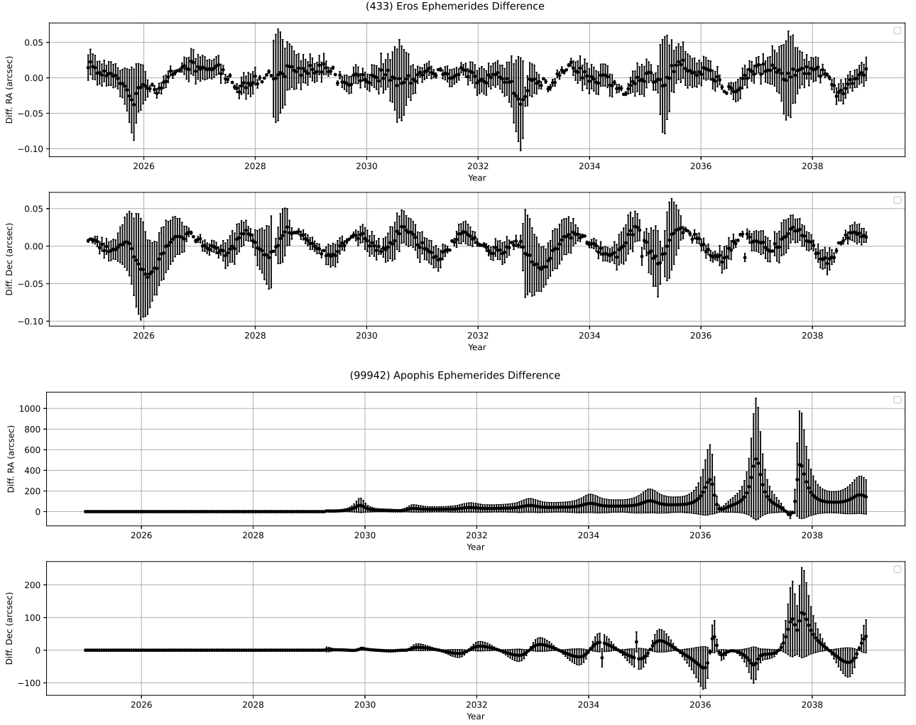
Figure 15. Differences between the celestial coordinates RA and Dec computed by Aegis and JPL Horizons, for asteroid (433) Eros (first and second panels) and (99942) Apophis (third and fourth two panels). Ephemerides as seen from the Geocenter are computed between 1 January 2025 and 1 January 2039, with a time-step of 15 days. Error bars refer to the 3\text{-}\sigma uncertainty in the corresponding element computed by Aegis, as obtained as a projection of the uncertainty ellipsoid on RA and Dec, respectively.
