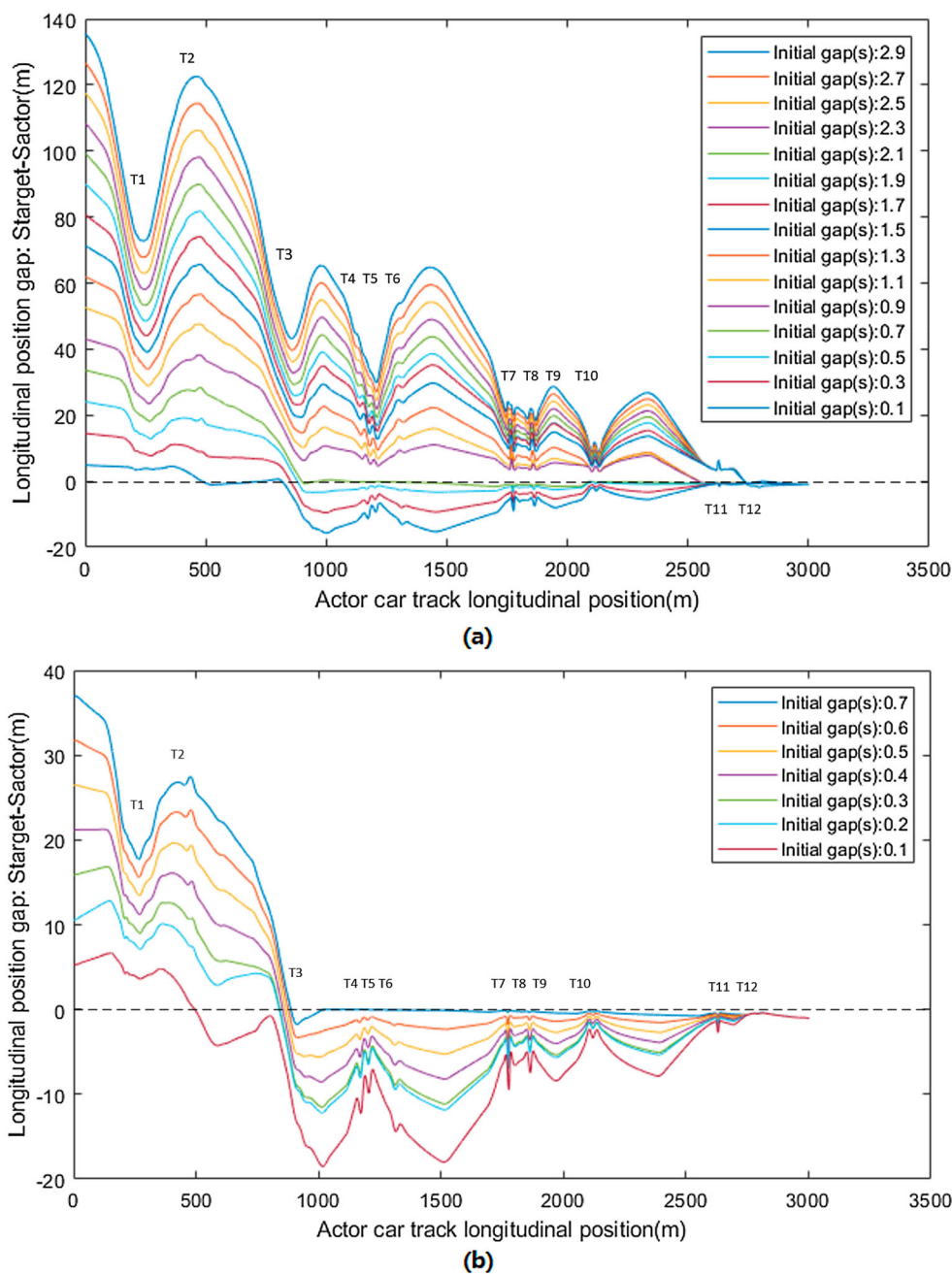
Figure 8. The relative position of the actor and target cars: (a) scenario S4 with target car energy allowance of 1.4kWh and (b) scenario S4 with target car energy allowance of 1.7kWh. Turn numbers are marked corresponding to Figure 4(a).
