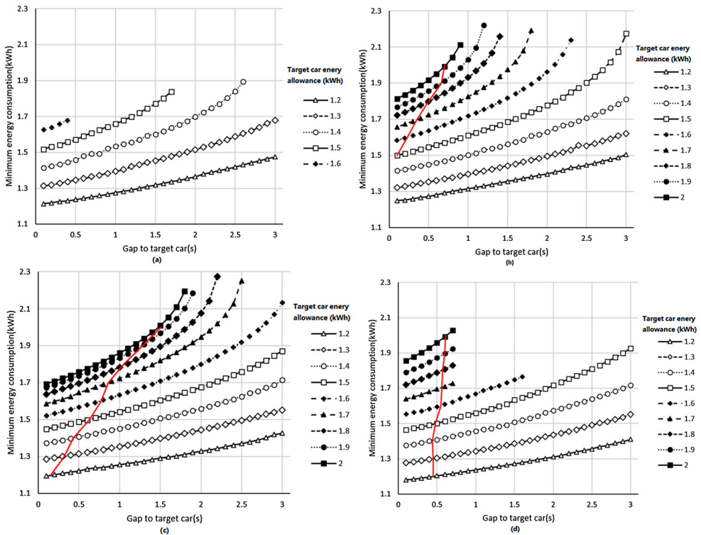
Figure 7. Minimum energy consumption for a successful overtaking lap: (a) scenario S1; (b) scenario S2; (c) scenario S3; (d) scenario S4. The red lines categorise the simulations into two groups. On the left-hand side, the actor car can overtake the target using less energy than the target car. The right-hand side is the opposite.
