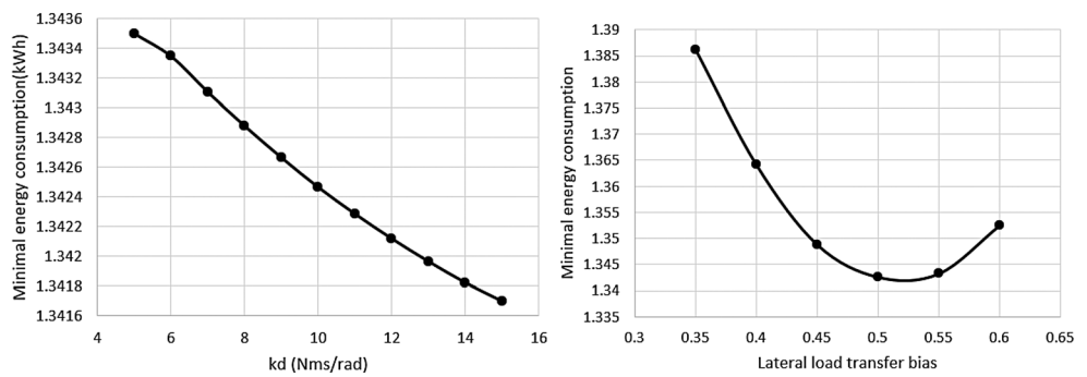
Figure D3. Minimum energy consumption sensitivity example (left) rotational damping coefficient of LSD (right) the lateral load transfer bias.
