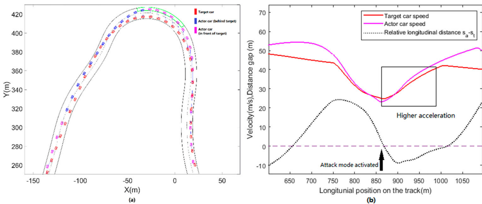
Figure 6. Overtaking at turn three: (a) car trajectories and (b) speed profile and relative position.
