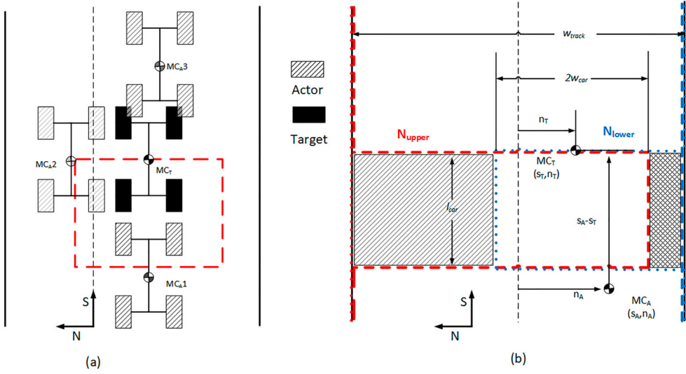
Figure 3. Collision exclusive zone.
