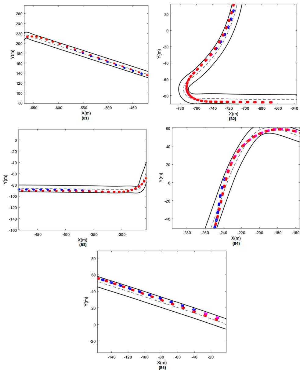
Figure C1. Overtaking trajectories at different positions of the track. B1: before turn seven, B2: before turn 10, B3: before turn 11, B4: before turn 12, B5: before finishing line, red block: target car, blue block: actor car before overtaking, purple block: actor car after overtaking.
