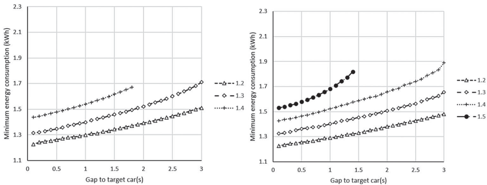
Figure D2. Minimum energy consumption for a successful overtaking lap on a slippery track condition (left) scenario S1 and (right) scenario S6.
