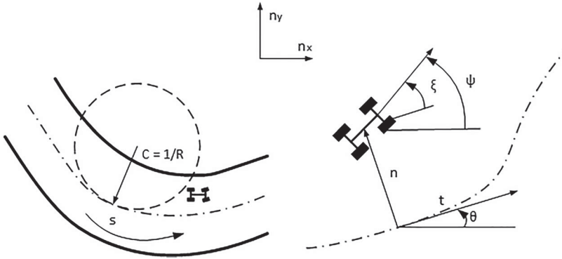
Figure A1. Track curvilinear coordinates.
