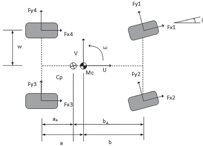
Figure A3. 7 DOF Vehicle model
