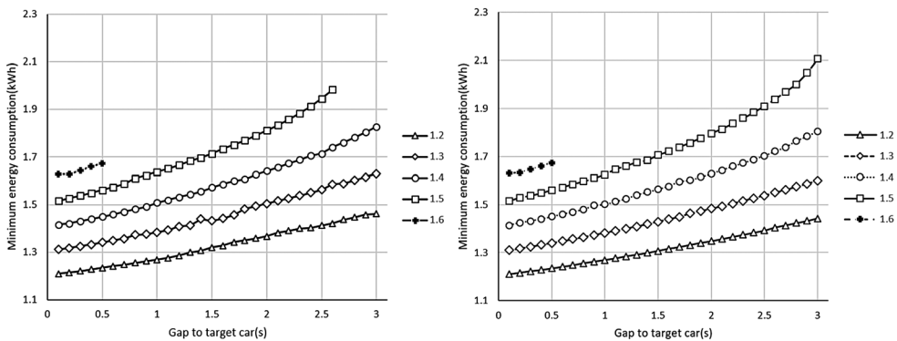
Figure D1. Minimum energy consumption for a successful overtaking lap (left) scenario S5 and (right) scenario S6.
