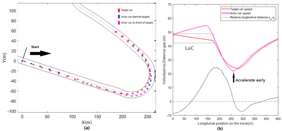
Figure 5. Overtaking at turn one: (a) car trajectories and (b) speed profile and relative position.
