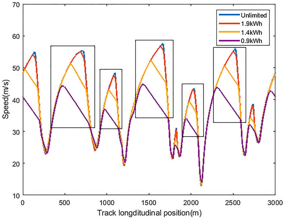
Figure 1. Speed profiles using different EPLs.
