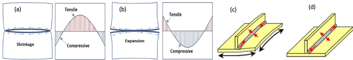
Fig. 2. The effect of tensile and compressive residual stresses along a longitudinal section of a weld (A Ohta et al., 1999) (Alghamdi and Liu, 2014).
