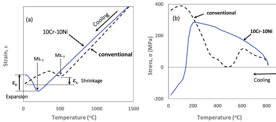
Fig. 4. The change of residual strain/stress with temperature for LTT and conventional weld wires: (a) strain and (b) stress (Ota et al., 2000) (A Ohta et al., 1999) (A Ohta et al., 1999) (Ota et al., 2001) (Ohta et al., 2003) (Miyata and Suzuki, 2015).
