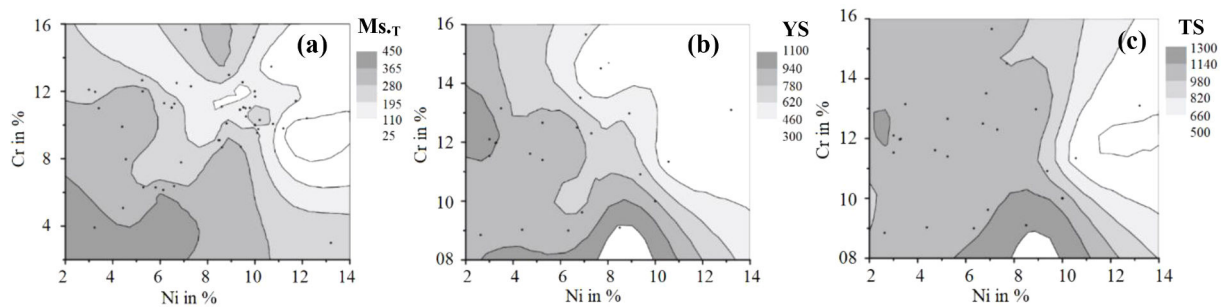
Fig. 19. The effects of increasing Cr-Ni on M_{s,T} , YS and TS of welding filler (Kromm, 2014).
