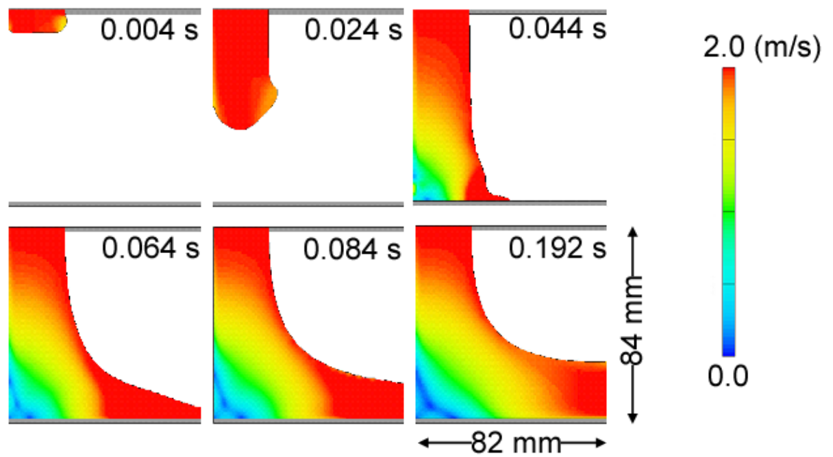
Figure 3. A series of frames for the 2D modelling result of the L5-junction V_i 2 I_o 24.
