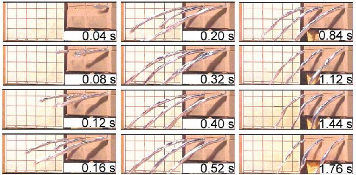
Figure 18 The trajectory method used for the estimation of the launch velocity V_o of the three streams issuing from the end of the 3 gates of the multiple-gate design.
