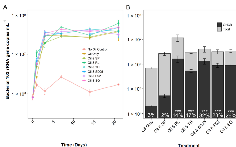
Figure 2. Bacterial 16S rRNA gene abundance (mean \pm SE, n = 3 ) over a 21 day period for total bacteria (A) and at day 1 only, for total bacteria and proportion (percentage figures) of obligate hydrocarbonoclastic bacteria (B). OHCB sequences are defined as from the genera: Alcanivorax , Cycloclasticus , Oleibacter , Oleispira , Thalassolituus . All microcosms contained seawater, nutrients, and oil (NSO-1 0.1% v/v ), and some also contained additional dispersants or biosurfactants (0.005% v/v ; 20:1 ratio of oil). Dispersant and biosurfactant codes are as follows: SP = sophorolipid, RL = rhamnolipid, TH = trehalolipid, SD25 = Superdispersant 25, F52 = Finasol OSR 52, and SG = Slickgone NS. Asterisks above percentage figures indicate significant differences in mean OHCB relative abundance compared to the oil-only control (** p < 0.001 ).
