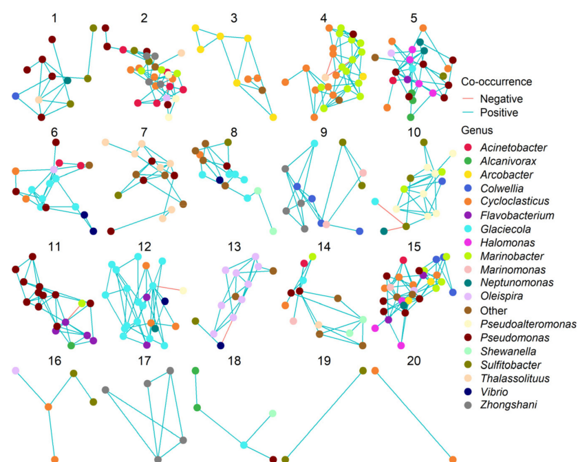
Figure 5. Network modules based on clustering of a SPIEC-EASI co-occurrence network formed of ASVs from bacterial genera associated with hydrocarbon degradation. Each point represents a single ASV, which are coloured according to their identity at the genus level (RDP classifier confidence >0.8). Blue edges represent positive co-occurrences between ASVs across the experiment, whereas red edges show negative co-occurrences.
