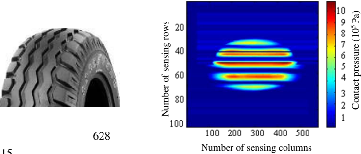
629 Fig. 15 630 A Goodyear 11.50/80-15.3 implement tyre at 2.18 tonne load and 4.1 \times 10^5 Pa inflation 631 pressure; left: tyre tread pattern; right: tyre contact pressure distribution ( 10^5 Pa) obtained 632 using the multi-point per sensel calibration with sensel selection (direction of travel: from 633 right to left)
