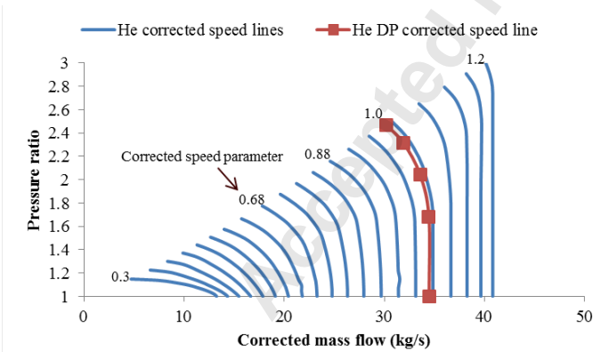
Fig. 6 Scaled component map for helium derived from the air working fluid reference map
