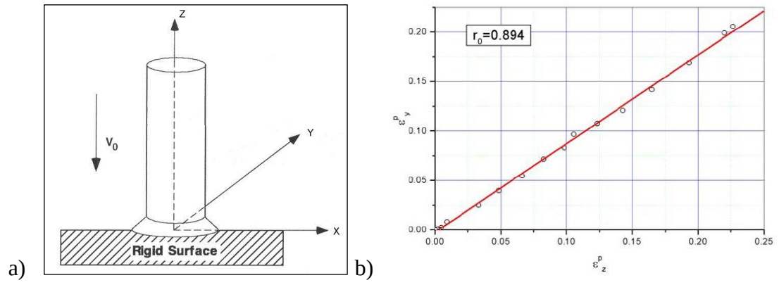
Figure 7 a) Taylor impact specimen and the reference coordinate system b) Lankford coefficient observed from Taylor test of AA7010 at (a) v = 200\text{m/s}
