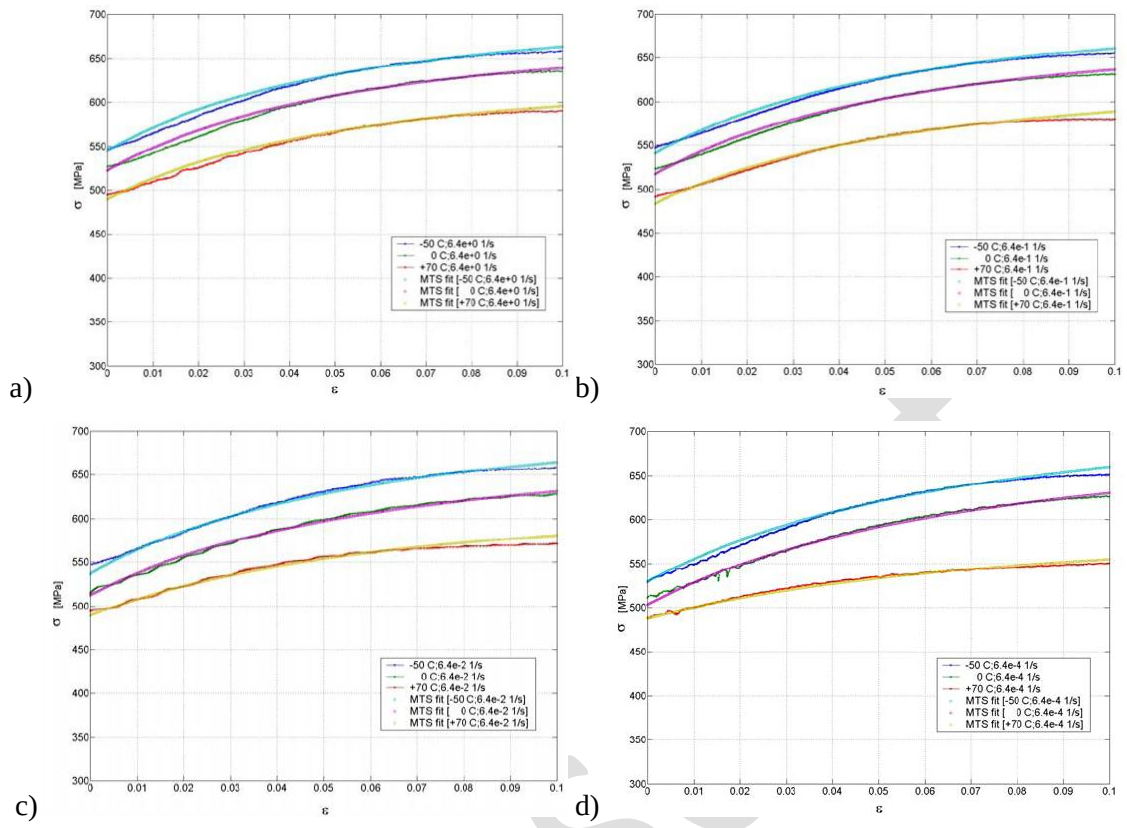
Figure 9 Experimental stress strain curves fitted with Mechanical Threshold Stress (MTS model) for the following strain rates: a) \dot{\epsilon} = 6.4 \times 10^0 \text{ s}^{-1} ; b) \dot{\epsilon} = 6.4 \times 10^{-1} \text{ s}^{-1} ; c) \dot{\epsilon} = 6.4 \times 10^{-2} \text{ s}^{-1} ; d) \dot{\epsilon} = 6.4 \times 10^{-4} \text{ s}^{-1}
