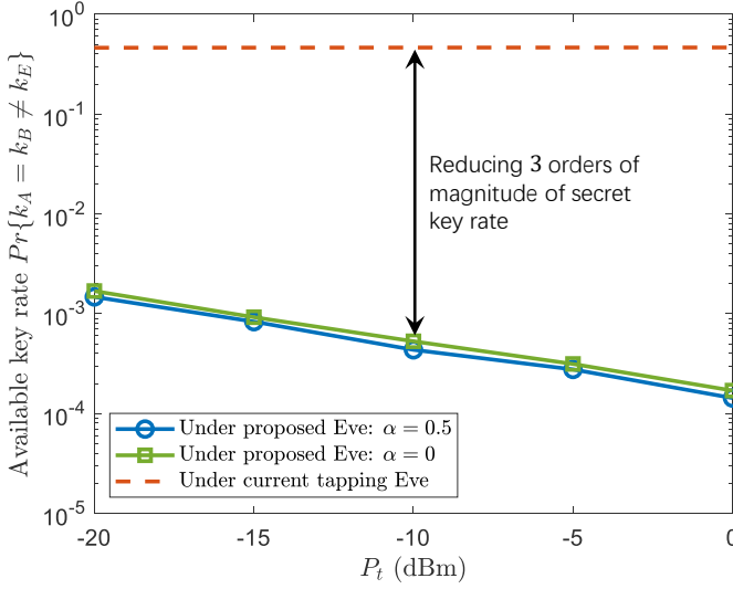
Fig. 7. Available key rate with two-way PL-SKG between Alice and Bob under our proposed Eve, i.e., Pr\{k_A = k_B \neq k_E\} . A three-order-of-magnitude reduction of the available key rate is obtained by our proposed Eve
