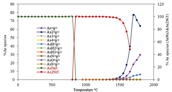
Fig. 3. Speciation of Arsenic.
