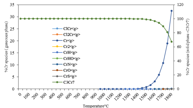
Fig. 2. Speciation of Chromium.
