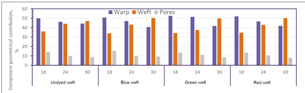
Fig. 4. Geometrical contribution of tested yarns in the case of plain weave (undyed warp, warp density = 30 ends/cm)
