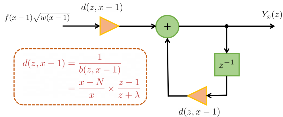
Figure 4. 1D digital filter structure to generate Y_x(z) based on Equation (29).
