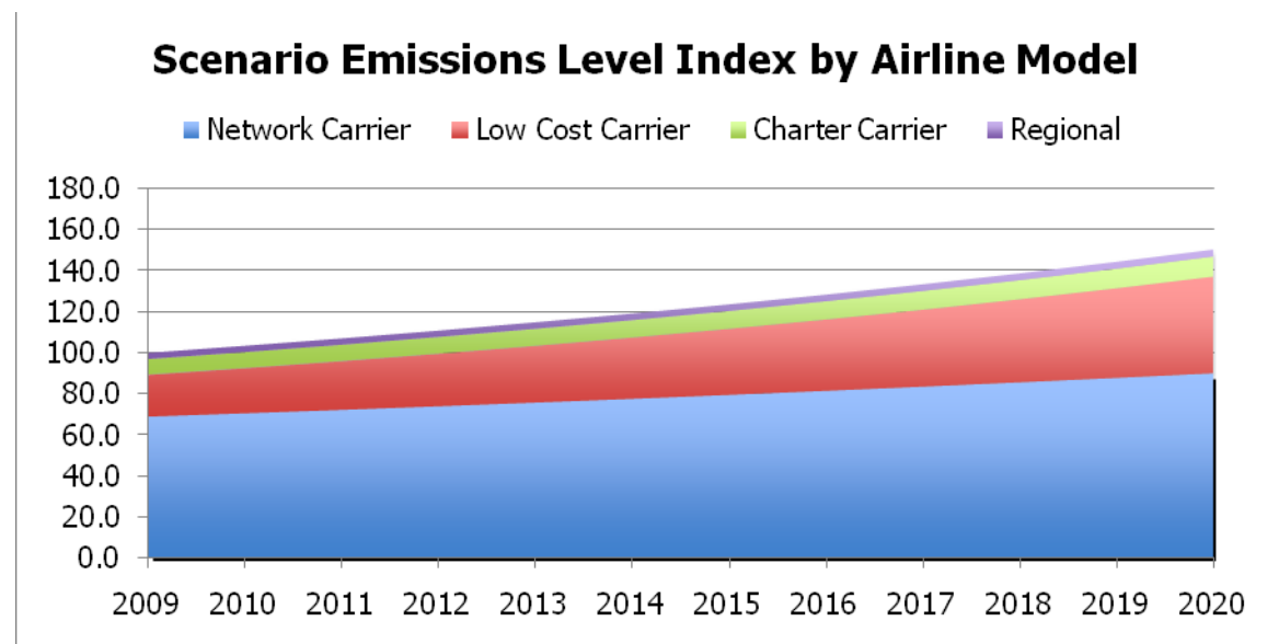
Figure 10: Total CO 2 Emissions Level Index by Airline Model (base case scenario)
