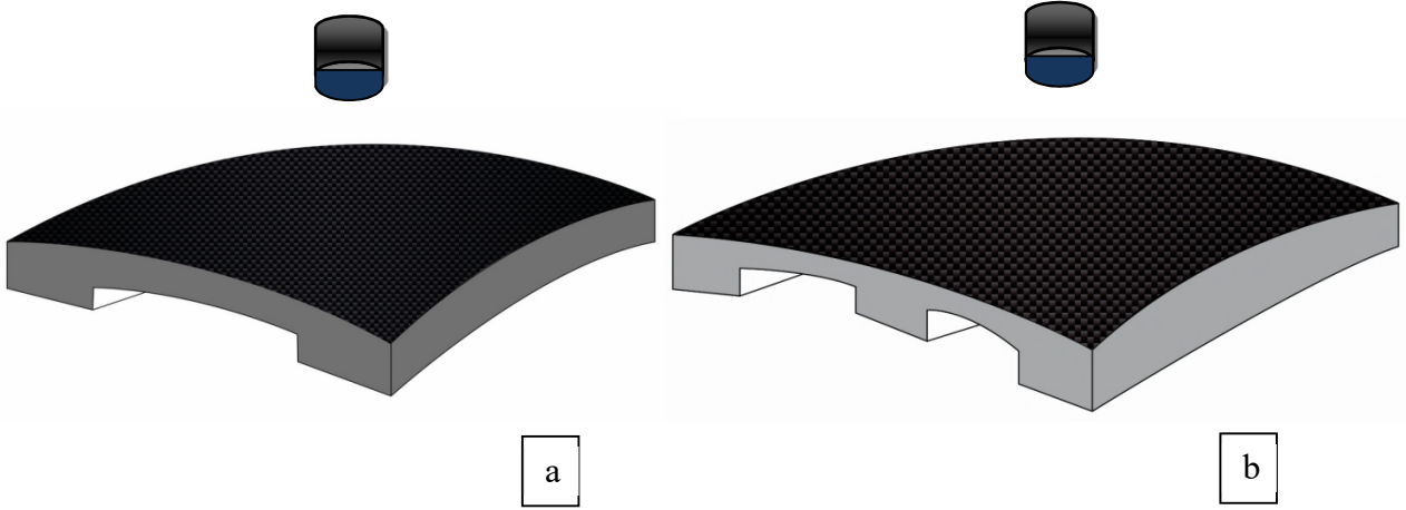
Fig. 1. The schematic curved composite plate with variable thickness (stiffness), a) three sectioned curved plate and b) five sectioned curved plate.
