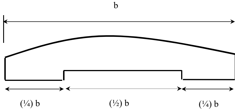
Fig. 5. Three sectioned curved composite plate with variable thicknesses in unequal widths.
