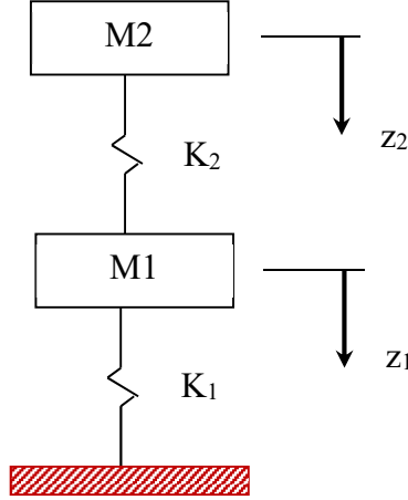
Fig. 2. Two-degrees-freedom of spring-mass system to model dynamic force.
