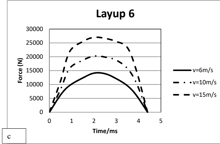
Fig. 11. Effect of impact velocity on five section variable thickness plate a) Layup 4 b) Layup 5 and c) Layup 6.
