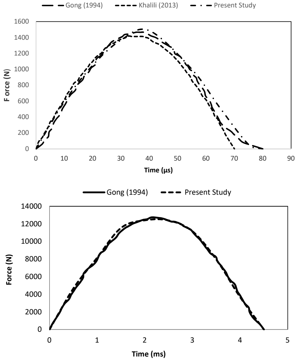
Fig. 3. a) Comparison of the force-time history for a) Steel plate and b) composite plate between the results of this work and results available in the literature.
