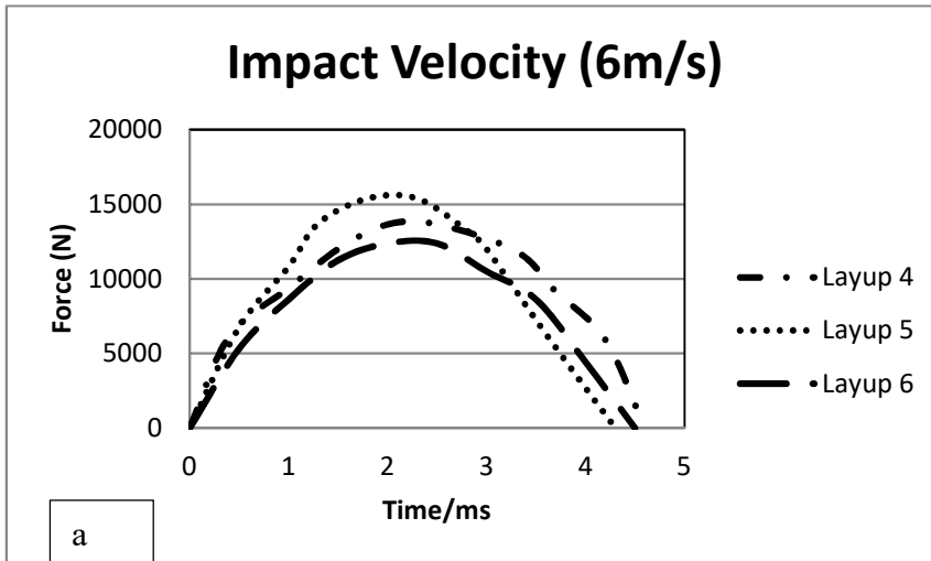
Fig 12. Effect of stacking sequence on three section variable thickness plate with unequal sections a) 6m/s b) 10m/s and c) 15m/s.
