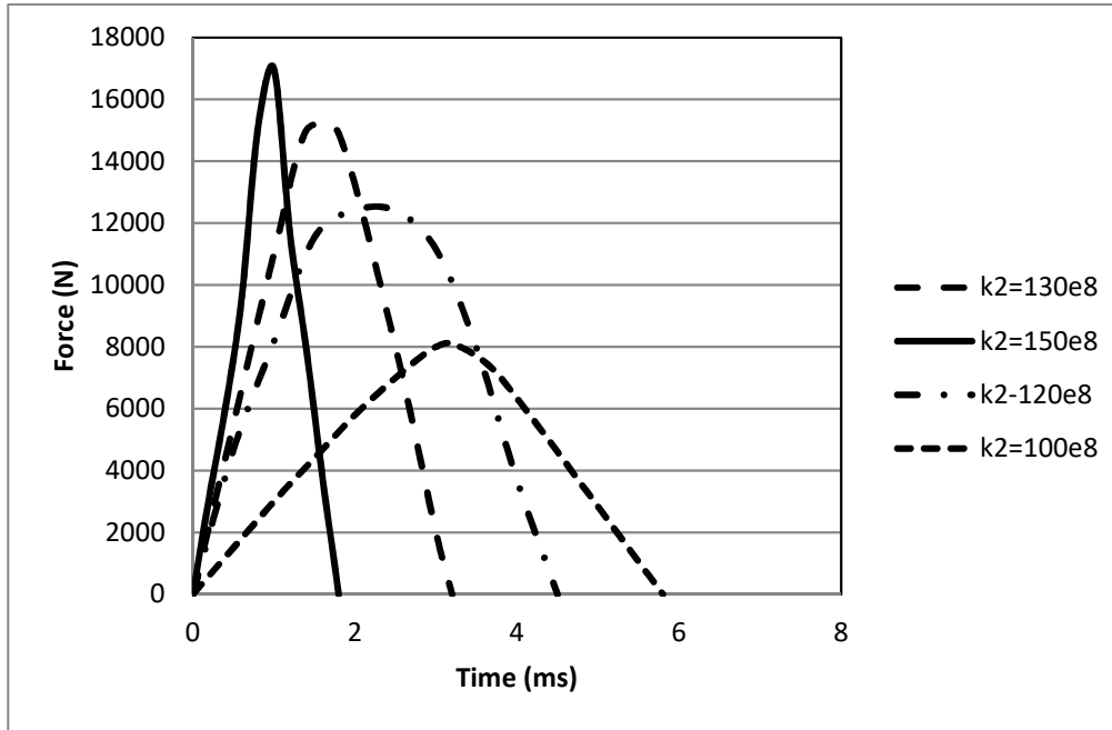
Fig. 7. Effect of contact stiffness on contact force history.
