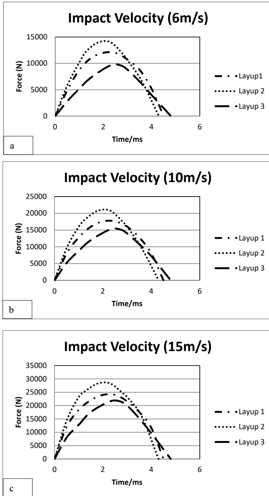
Fig. 8. Effect of stacking sequence on the three sectioned plate with variable thicknesses a) 6m/s, b) 10m/s and c) 15m/s.
