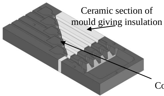
a) large ceramic section insulated mould
