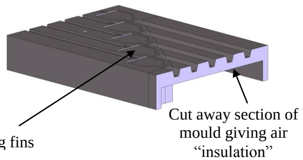
b) cut-away section insulated mould
