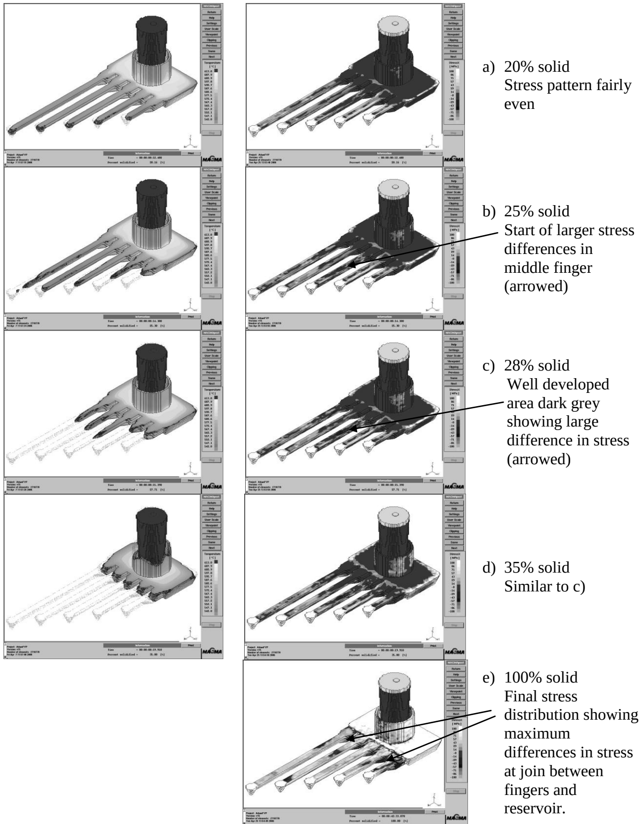
Solidification pattern Stress Figure 6: Predicted solidification sequence for the original 5 fingered die and stresses developed within the fingers at different times during the solidification
