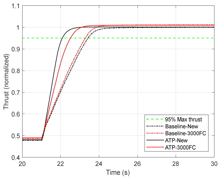
(b) Thrust
