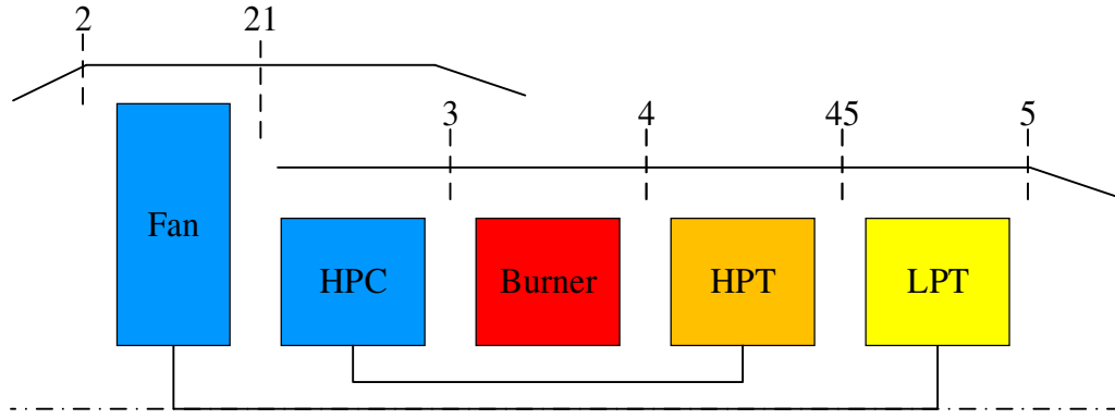
Fig. 1 Schematic of the examined dual-spool turbofan engine
