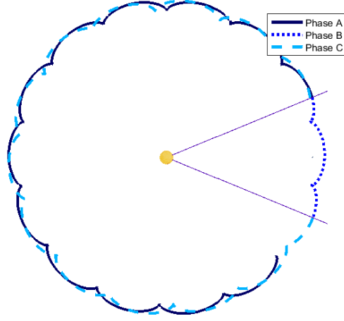
Fig. 5: Phases of the capture trajectory with an Earth-resonant encounter
