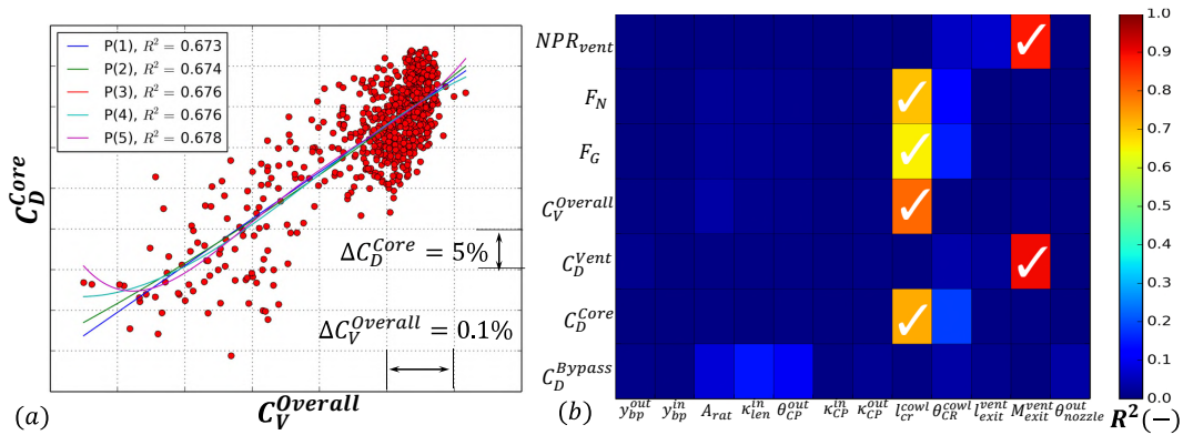
Figure 7. Polynomial regression analysis: (a) correlation process between C_V^{Overall} and C_D^{Core} , (b) Hinton visualisation of 5^{th} -order polynomial regression applied throughout entire design space
