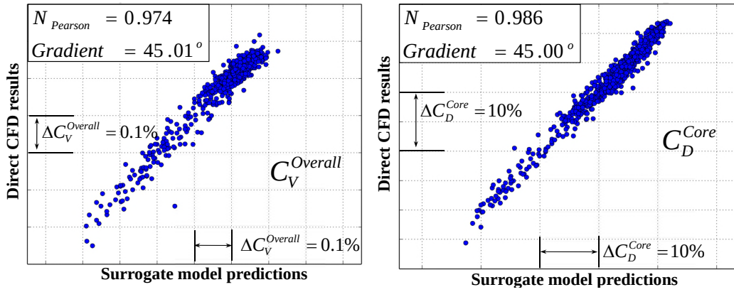
Figure 8. LOO cross-validation applied to the structured surrogate models for for: (a) C_V^{Overall} and (b) C_D^{Core}
