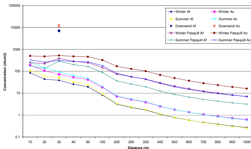
Figure 3. The influence of season and meteorological data on modelled predicted concentrations of A. fumigatus (Af) and actinomycetes (Ac).
