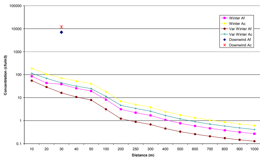
Figure 1. Modelled predicted concentrations of A. fumigatus (Af) and actinomycetes (Ac) for the winter, showing both constant emissions and intermittent emissions.
