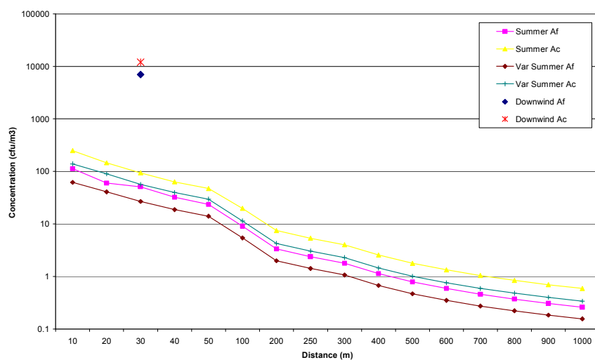
Figure 2. Modelled predicted concentrations of A. fumigatus (Af) and actinomycetes (Ac) for the summer, showing both constant emissions and intermittent emissions.
