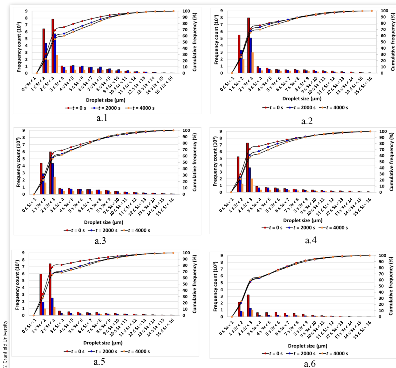
FIGURE 4 Water droplet size population with respect to time for each fuel for Cases a.1-a.6.
