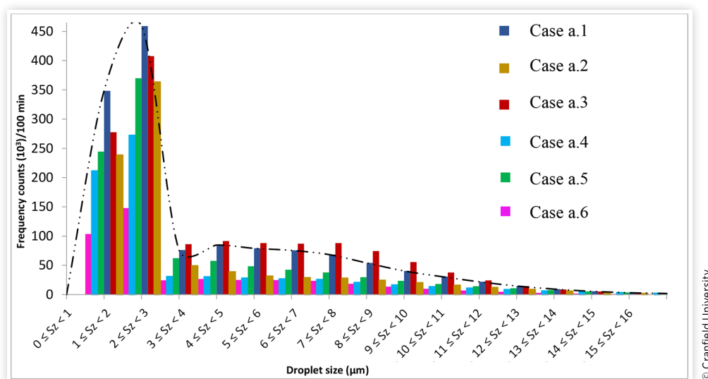
FIGURE B.1 Frequency distribution of the different size water droplets after 100 min settling for the six aviation fuels explored in this work.
