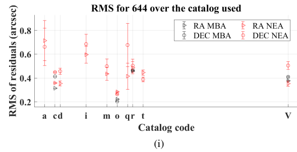
Figure 7. RMS of residuals over the catalogues of observation. The plots for Main Belters and Near-Earth asteroids are plotted differentiating between the residuals for Right Ascension and Declination.
