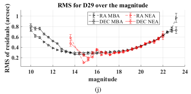
Figure 5. RMS of residuals over the magnitudes of observation. The plots for Main Belters and Near-Earth asteroids are plotted differentiating between the residuals for Right Ascension and Declination.
