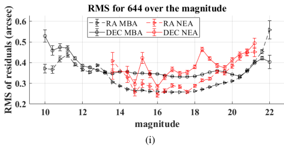
Figure 5. RMS of residuals over the magnitudes of observation. The plots for Main Belters and Near-Earth asteroids are plotted differentiating between the residuals for Right Ascension and Declination.
