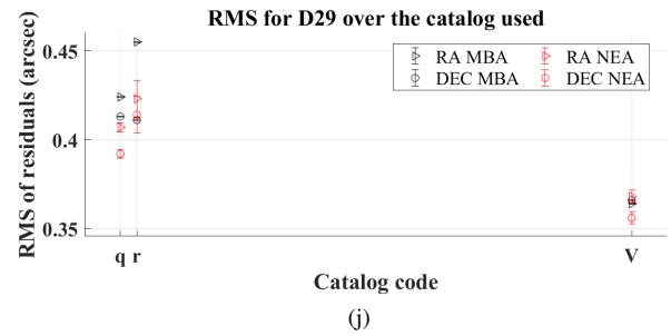
Figure 7. RMS of residuals over the catalogues of observation. The plots for Main Belters and Near-Earth asteroids are plotted differentiating between the residuals for Right Ascension and Declination.
