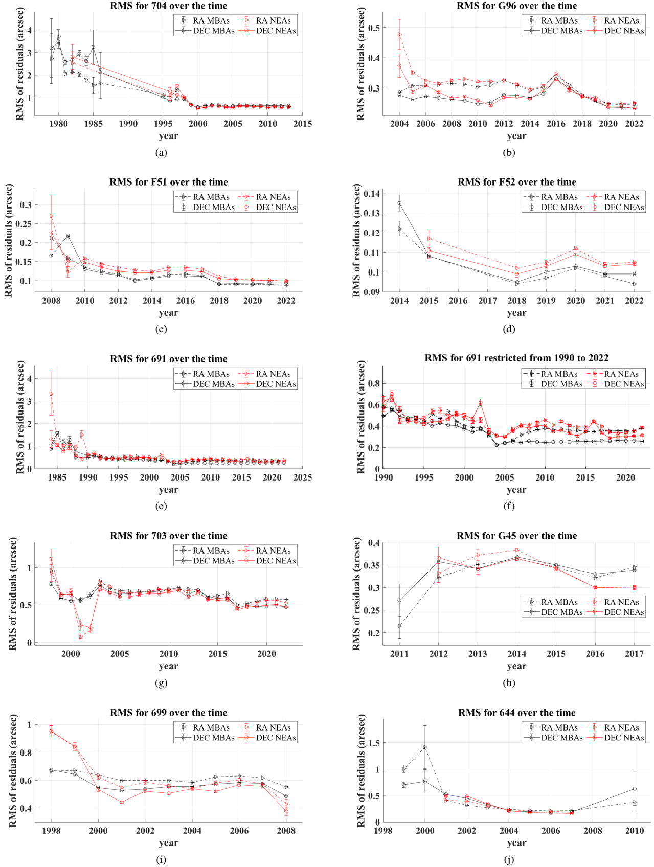
Figure 3. RMS of residuals over the years of observation for the considered stations. The plots for Main Belters and Near-Earth asteroids are plotted differentiating between the residuals for Right Ascension and Declination.
