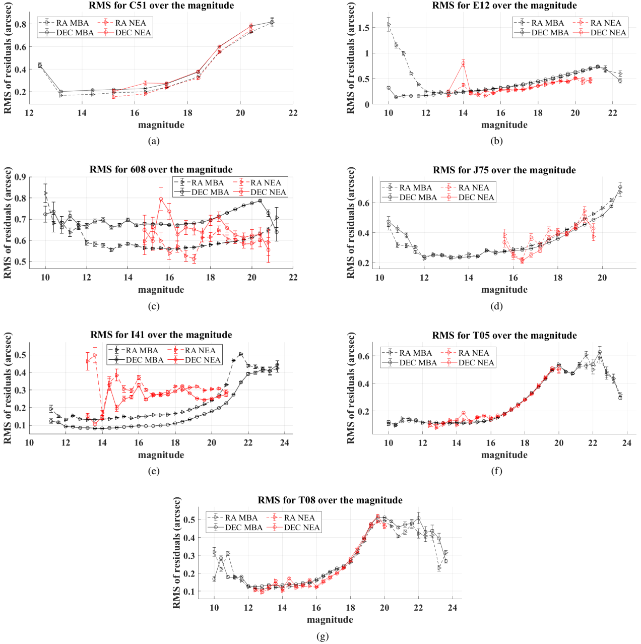
Figure 6. RMS of residuals over the magnitudes of observation. The plots for Main Belters and Near-Earth asteroids are plotted differentiating between the residuals for Right Ascension and Declination.
