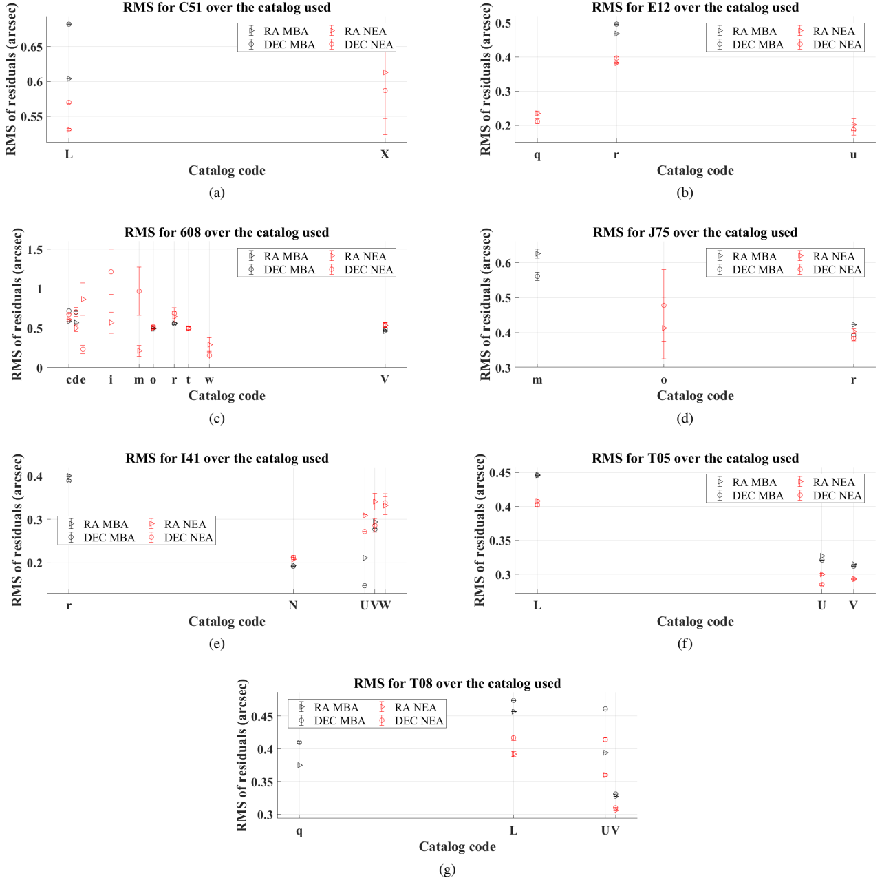
Figure 8. RMS of residuals over the catalogues of observation. The plots for Main Belters and Near-Earth asteroids are plotted differentiating between the residuals for Right Ascension and Declination.
