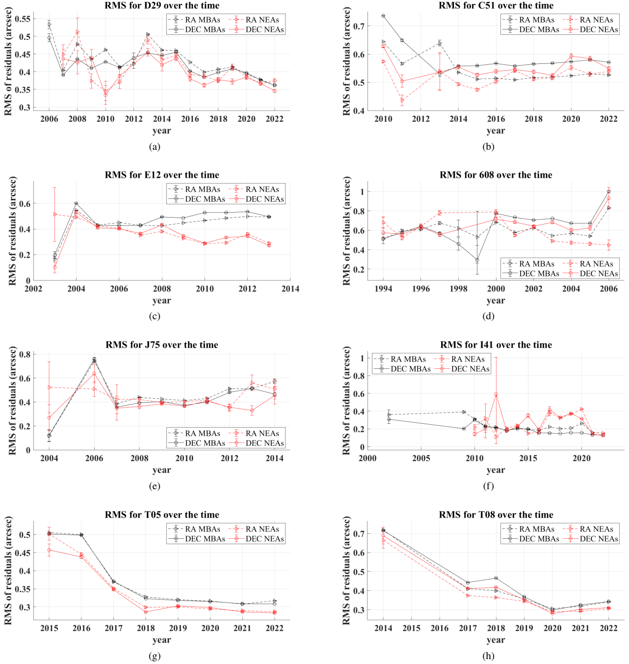
Figure 4. RMS of residuals over the years of observation for the considered stations. The plots for Main Belters and Near-Earth asteroids are plotted differentiating between the residuals for Right Ascension and Declination.
