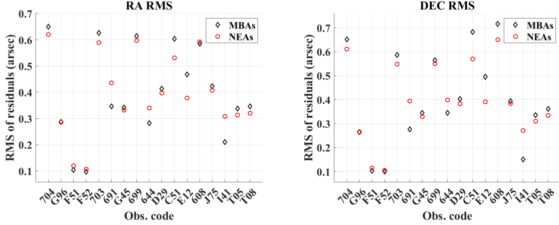
Figure 1. RMS of residuals in RA (left panel) and DEC (right panel) for all the stations, considering the values for NEAs and MBAs
