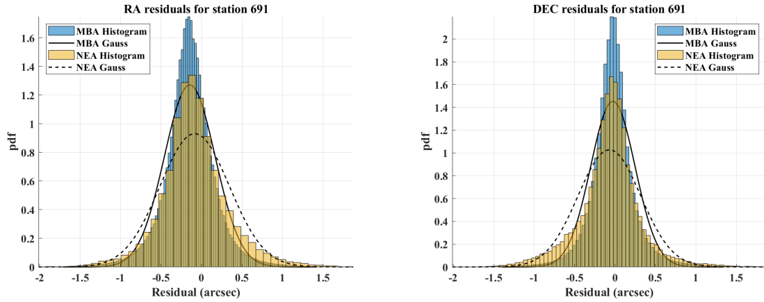
Figure 2. Probability density function (pdf) of the distribution of the residuals for station 691 in Right Ascension (left panel) and Declination (right panel). The histogram and the Gaussian Normal Distribution are represented superimposed for the residuals of MBAs and NEAs observations distinctly.
