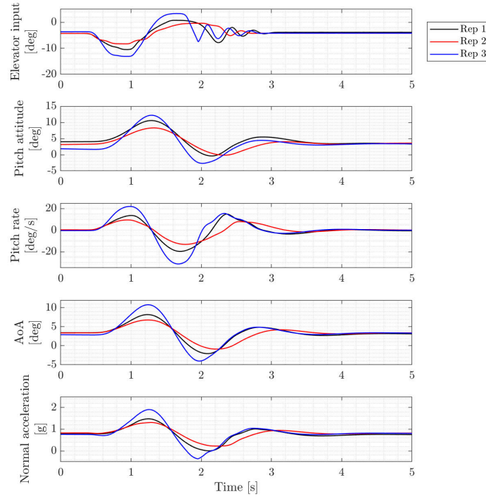
Fig. 6 Time histories of the SPPO response for configuration A1.
