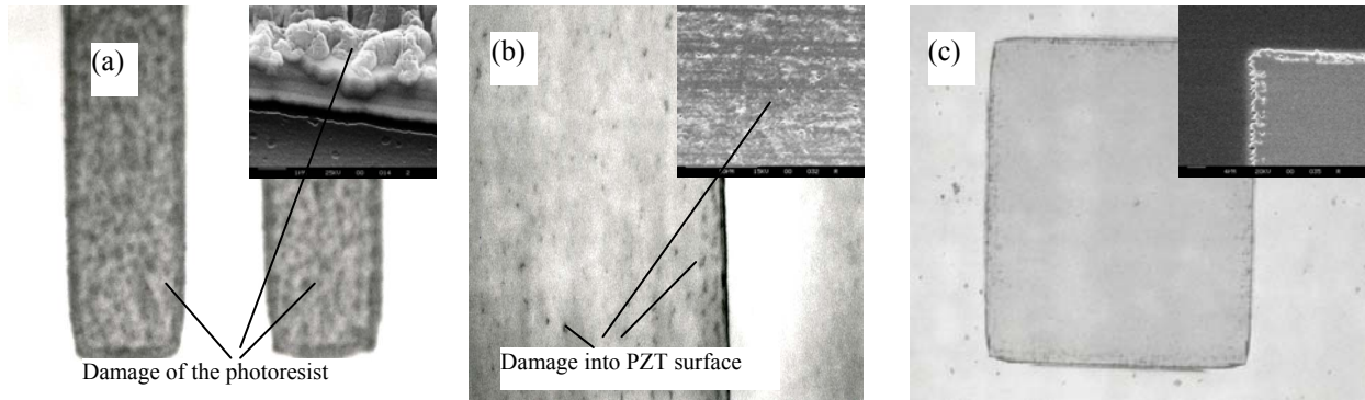
Figure 4: PZT pattern processed at RF power of 200W and 175W (the inner graphs are the SEM images) (a) damaged photoresist; (b) the damage deepened into the PZT surface; (c) undamaged PZT surface
