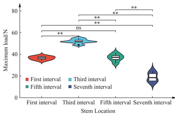
Figure 14 Prediction and loading of internode load of stem
