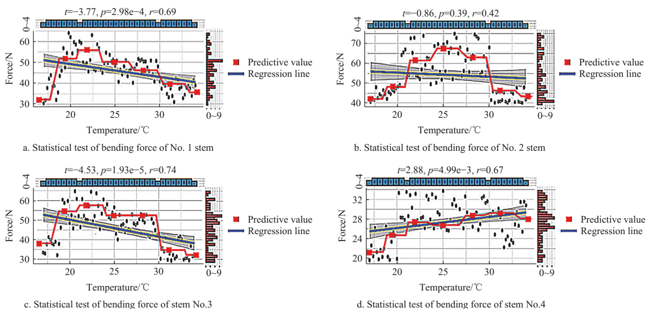
Figure 22 Statistics and t-test of the bending force of No.1-4 stems at 16°C-34°C
